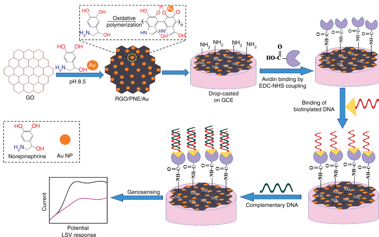
Figure 8. Schematic diagram of rGO/PNE/Au nanocomposites synthesis and detection procedure for MTB DNA. Reproduced from (81), Copyright (2022), with permission from Elsevier. rGO/PNE MTB, Mycobacterium tuberculosis; rGO, reduced graphene oxide; PNE, polynorepinephrine.
