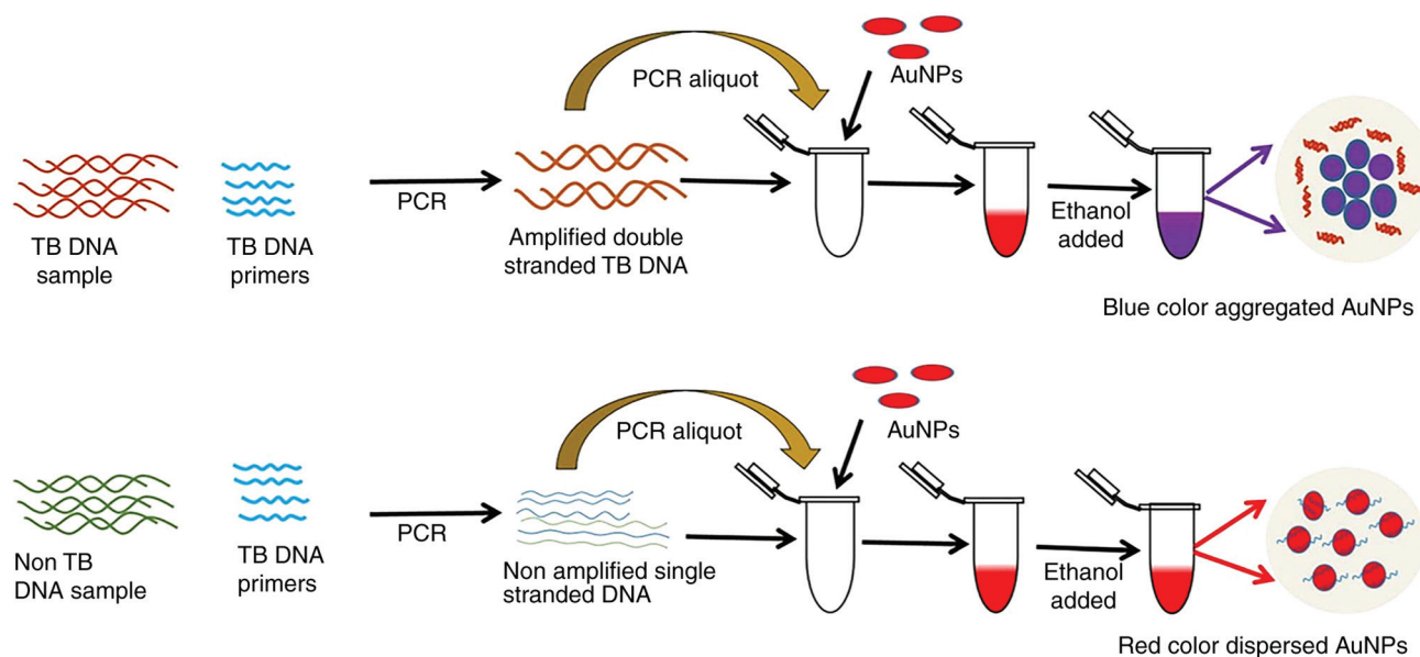
Figure 2. AuNPs-based colorimetric detection of TB DNA Schematic diagram: Two PCR tubes were made using TB primers and PCR mix. The TB DNA template was placed in one tube and the other tube without the TB DNA template. After PCR, AuNPs and ethanol were added. The tube without the DNA template stayed red, while the tube with TB DNA turned purple. Reproduced from (32), Copyright (2023), with permission from Royal Society of Chemistry. AuNPs, gold nanoparticles; TB, tuberculosis.
