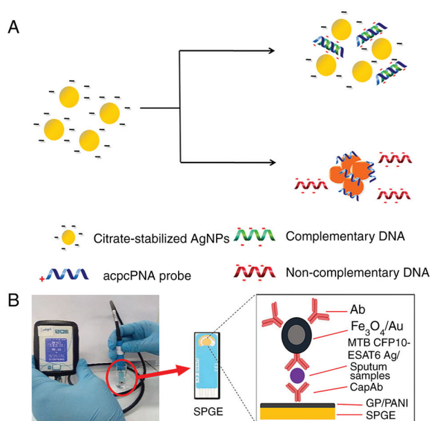
Figure 4. Procedure for acpcPNA-induced AgNP aggregation. (A) AgNPs were initially well dispersed by the negatively charged electrostatic repulsion. Positively charged acpcPNA shielded them from electrostatic repulsion, causing silver particles to aggregate and a color reaction to occur. When complementary DNA was present, the specific PNA-DNA interaction replaced the PNA-AgNPs interaction, forming negatively charged PNA-DNA double strands that depolymerized the nanoparticles. In the case of non-complementary DNA, the nanoparticles did not depolymerize and no color change occurred. Reproduced from (54), Copyright (2017), with permission through Creative Commons public use license from Teengam P et al. , American Chemical Society. (B) Schematic of CFP10-ESAT6 detection using the portable electrochemical reader. Sputum sample analysis was performed locally with the modified SPGE (circled in red) and a portable reader. Following GP/PANI modification of SPGE, the CapAb was immobilized on its surface to capture the target antigen and the Ab-loaded Fe 3 O 4 /Au particle bound to the target and amplified the detection signal. Reproduced from (41), Copyright (2021), with permission from Springer Nature. acpcPNA, PNA with a positively charged lysine modification at its C-terminus; AuNPs, gold nanoparticles; PNA, peptide nucleic acid; CFP10, culture filtrate antigen, 10 kDa; ESAT-6, early secreted antigenic target-6; SPGE, screen-printed gold electrode; GP/PANI, graphene/polyaniline; CapAb, capture antibody; MTB, Mycobacterium tuberculosis.
