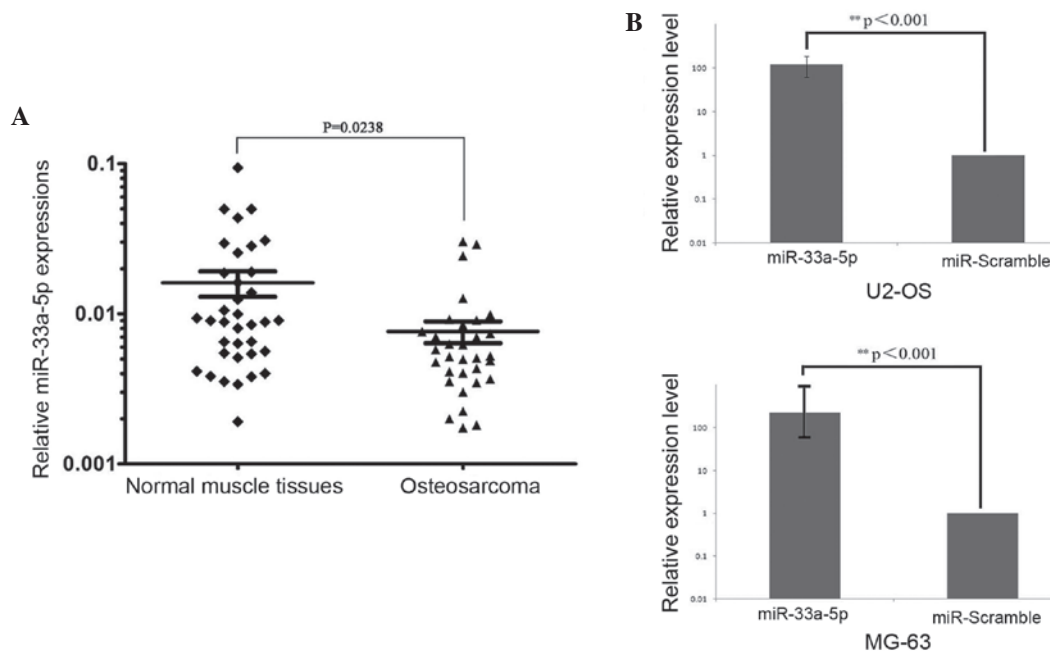
Figure 2. miR-33a-5p expression is decreased in OS cells and tissues. (A) Relative expression of miR-33a-5p was evaluated by TaqMan (RT-qPCR). Human normal muscle RNAs were used as controls. miR-33a-5p expression was downregulated in OS tissues. (B) Confirmation of overexpression of miR-33a-5p in transfected cell lines by real-time PCR. OS cell lines U-2OS and MG-63 were transfected with miR-33a-5p precursor and miR-Scramble control, and the relative expression of miR-33a-5p was assessed by RT-qPCR. Values are presented as the mean \pm standard deviation. miR, microRNA; RT-qPCR, reverse transcription-quantitative polymerase chain reaction; OS, osteosarcoma.
