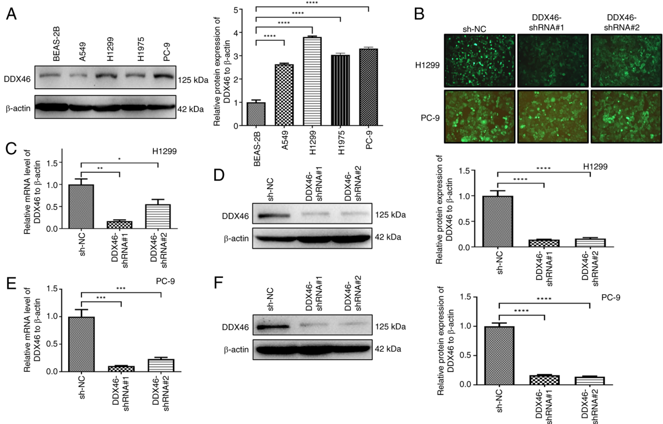
Figure 3. Expression of DDX46 in several cell lines and the effect of silencing DDX46 in vitro . (A) DDX46 protein levels in BEAS-2B, A549, H1299, H1975, and PC-9 cell lines. (B) The knockdown DDX46 lentiviral vector was transfected into H1299 and PC-9 cells, with the intensity of the green fluorescence signal serves as an indicator of the efficiency of the corresponding lentivirus transfection (magnification, x200). The effect of silencing DDX46 in H1299 cells was assessed using (C) RT-qPCR and (D) western blotting, and the effect of silencing DDX46 in PC-9 cells was evaluated using (E) RT-qPCR and (F) western blotting. *P<0.05; **P<0.01; ***P<0.001; ****P<0.0001. DDX46, DEAD-box 4; RT-qPCR, reverse transcription-quantitative PCR; ns, no significance; NC, negative control; shRNA, short hairpin RNA.
