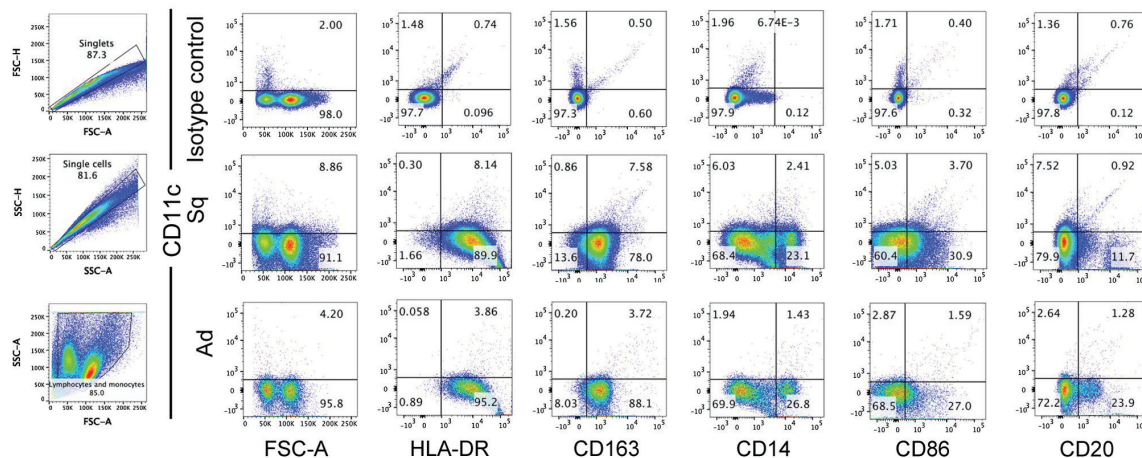
Figure S1. Flow cytometry analysis of tumour infiltrating CD45 + cells in patients with non-small cell lung cancer. Lymphocytes and monocytes in single cells were gated. Most tumour infiltrating CD45 + cells were HLA-DR positive. Many CD11c + cells were CD163 positive and CD20 negative. The CD11c + subset contained cells positive and negative for CD14 and CD86. Sq; squamous cell carcinoma, Ad; adenocarcinoma.
