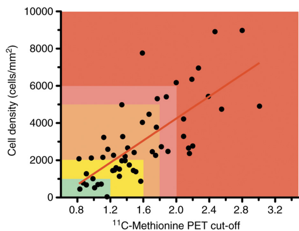
Figure S1. Correlation of glioma cell density and MET uptake on PET. Tumor cell density is plotted as a function of the tumor-to-normal tissue ratio of MET accumulation. A linear regression analysis was performed. These two factors showed a positive correlation ( P < 0.0001 ) with a Pearson's correlation r value of 0.72. PET, positron emission tomography.
