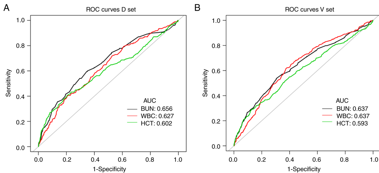
Figure S2. ROC curves of three risk predictors, namely the BUN level, WBC count and HCT level, in our stepwise model in the (A) training and (B) validation cohorts. WBC, white blood cells; BUN, blood urea nitrogen; HCT, hematocrit; ROC, receiver operating characteristic; AUC, area under the ROC curve.
