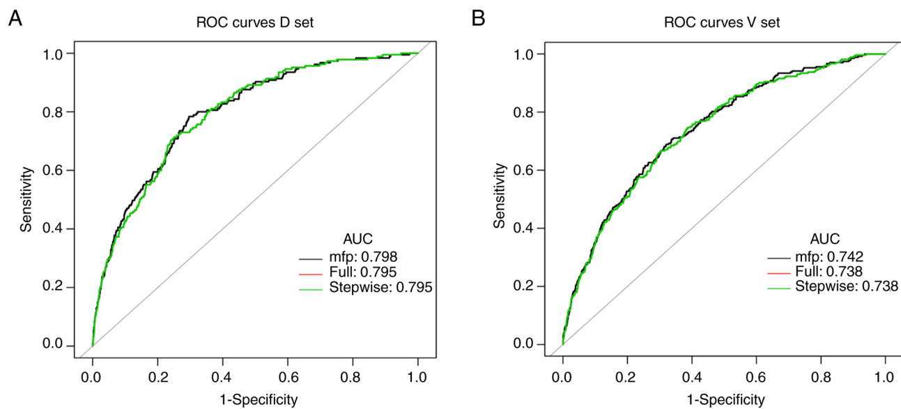
Figure S1. AUCs of the three models in the (A) training (D set) and (B) validation (V set) cohorts. ROC, receiver operating characteristic; AUC, area under the ROC curve; MFP, multivariable fractional polynomial.
