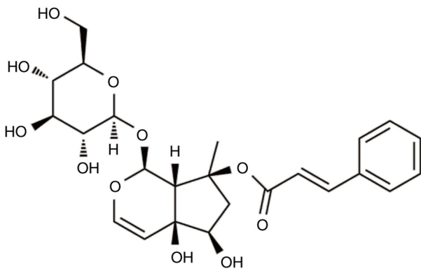
Figure 1. Chemical structural formula of harpagoside.
