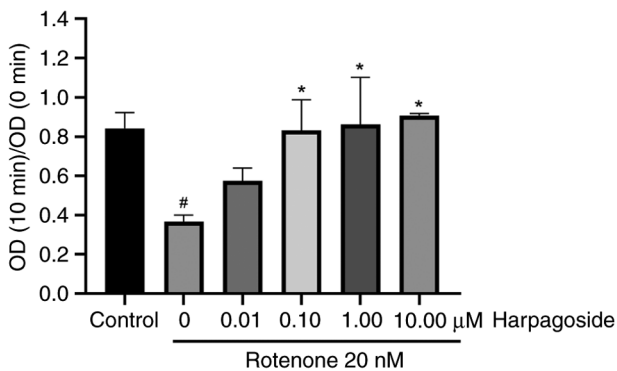
Figure 4. Effects of harpagoside on rotenone-induced mitochondrial swelling. Data are expressed as mean \pm standard error of the mean (n=3). #P<0.05 vs. Control; *P<0.05 vs. Model group. OD, optical density; prot, protein.
