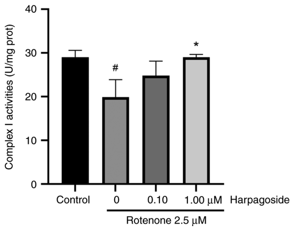
Figure 3. Effects of harpagoside on rotenone-induced mitochondrial complex I activity. Data are expressed as mean \pm standard error of the mean (n=3). #P<0.05 vs. Control; *P<0.05 vs. Model group.
