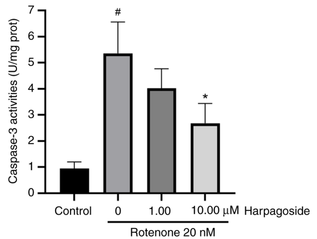
Figure 5. Effects of harpagoside on rotenone-induced caspase 3 activities. Data are expressed as mean \pm standard error of the mean (n=3). #P<0.05 vs. Control; *P<0.05 vs. Model group. Prot, protein.
