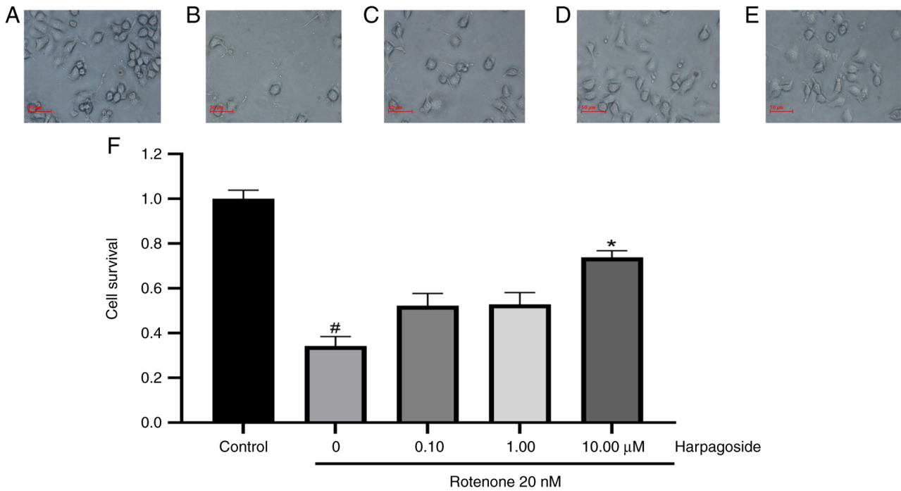
Figure 2. Protective effects of harpagoside on rotenone-induced effects in N2A cells. Data are expressed as mean \pm standard error of the mean (n=4). Representative image of N2A cell cultures under a light microscopy. (A) Control group, (B) Rotenone-treated group, Group treated with rotenone and (C) 0.1, (D) 1 or (E) 10 \mu mol/l harpagoside respectively. (F) Cell Survival Rate. #P<0.05 vs. Control; *P<0.05 vs. Model group.
