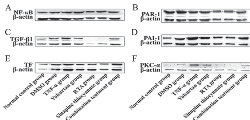
Figure 3. Western blots of inflammation and coagulation factors (A) NF- \kappa B, (B) PAR-1, (C) TGF- \beta 1, (D) PAI-1, (E) TF and (F) PKC- \alpha in TNF- \alpha mediated vascular endothelial cells. Seven lanes indicate the following groups, respectively: Normal control, DMSO, TNF- \alpha , valsartan, RTA, sinapine thiocyanate and combination treatment. NF- \kappa B, nuclear factor- \kappa B; PAR-1, protease-activation receptors; TGF- \beta 1, transforming growth factor- \beta 1; PAI-1, plasminogen activator inhibitor; TF, tissue factor; PKC- \alpha , protein kinase C; TNF- \alpha , tumor necrosis factor- \alpha ; DMSO, dimethylsulfoxide; RTA, rhynchophylla total alkaloids.
