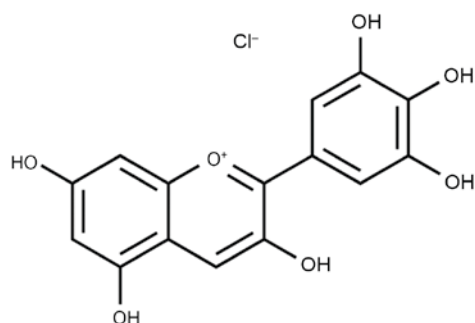
Figure 1. Chemical structure of delphinidin.
