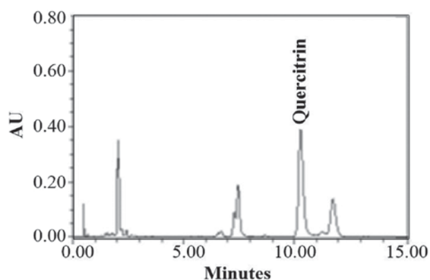
Figure 6. UPLC profile of CIEE. Chromatogram for the analysis of compounds isolated from CIEE. UPLC, Ultra pressure liquid chromatography; CIEE, ethanol extract of Chrysanthemum indicum L.
