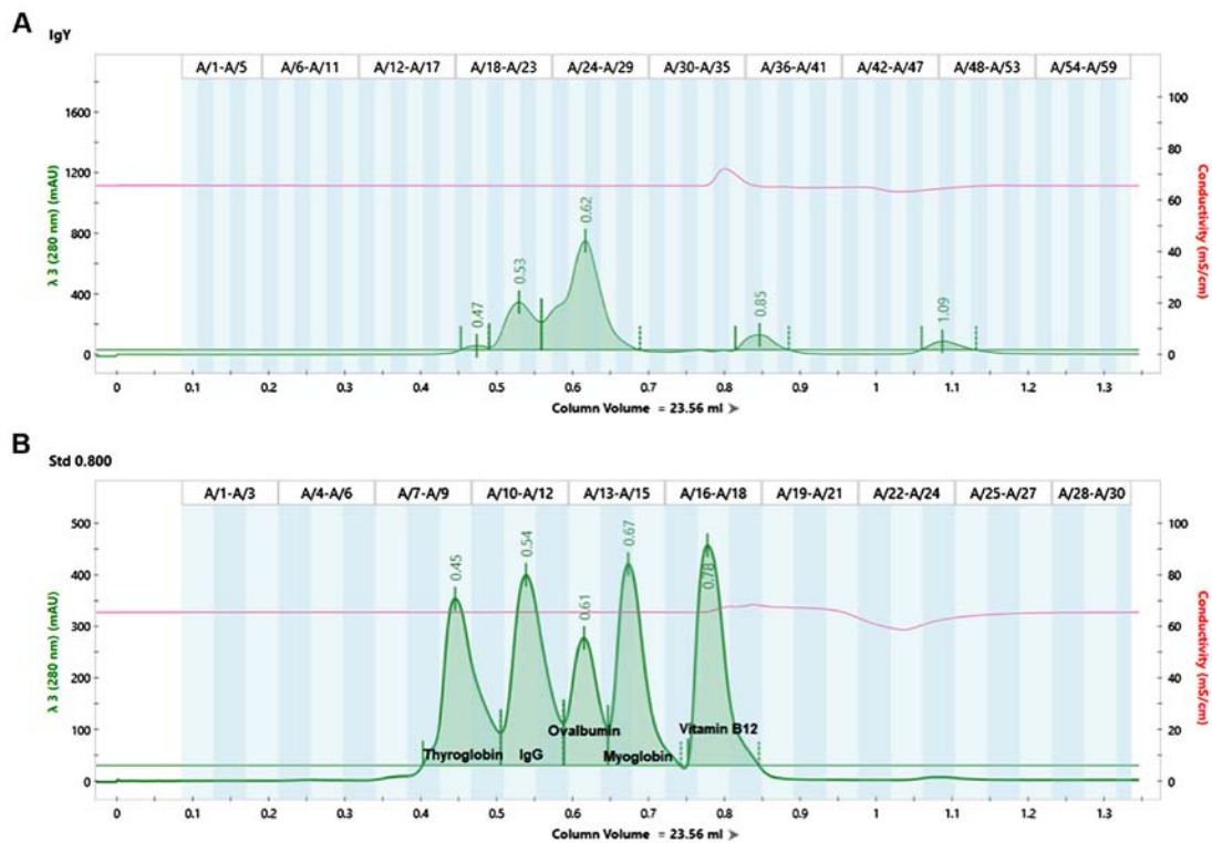
Figure 1. NGC Chromatograms of IgY extract isolated from hen egg yolk in comparison to standard protein cocktail. (A) Hen yolk egg IgY extract at 1 mg/ml concentration; (B) Standard protein cocktail for molecular weight identification. Column - size exclusion ENrich SEC 650, PBS elution, flow at 0.8 ml/min, absorbance registered 280 nm. IgY, immunoglobulin Y.
