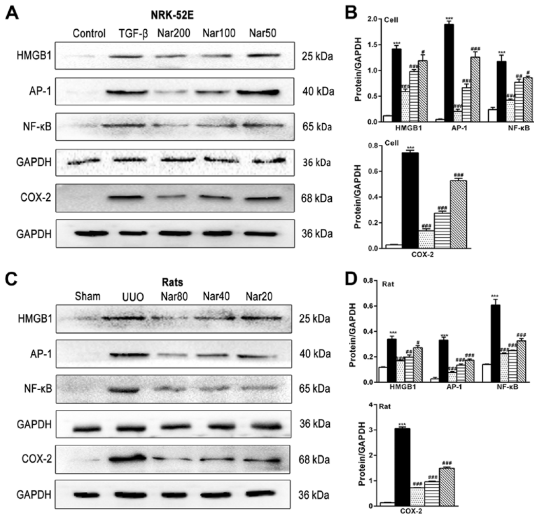
Figure 8. Effects of naringin on the expression of HMGB1, AP-1, NF-κB and COX-2 in NRK-52E cells and rat kidneys. (A) Effect of naringin on HMGB1, AP-1, NF-κB and COX-2 in NRK-52E cells. (B) Quantitative analysis of the protein expression of HMGB1, AP-1, NF-κB and COX-2 in NRK-52E cells. (C) Effect of naringin on HMGB1, AP-1, NF-κB and COX-2 in rat kidneys. (D) Quantitative analysis of the protein expression of HMGB1, AP-1, NF-κB and COX-2 in rat kidneys. Data is presented as mean ± SD (n=6). ***P<0.001 vs. Control; #P<0.05, ##P<0.01, ###P<0.001 vs. UUO or TGF-β. Nar, naringin; UUO, unilateral ureteral obstruction; HMGB-1, high-mobility group protein B1; COX-2, cyclooxygenase-2; AP-1, activator protein-1; TGF-β, transforming growth factor-β.
