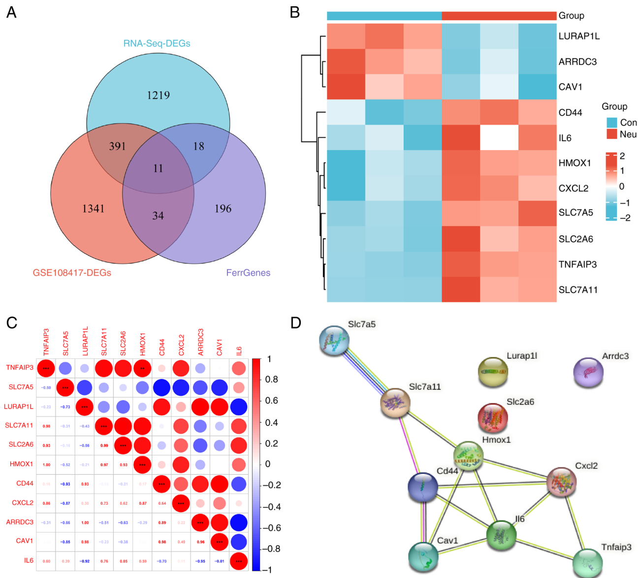
Figure 6. Analysis of ferroptosis-associated genes in neutropenic asthmatic mice. (A) Venn diagram representing the intersection between DEGs from RNA-seq and GSE108417 datasets, with a focus on ferroptosis-related genes. (B) Heatmap depicting ferroptosis-associated genes in neutropenic asthmatic mice. Red and blue stand for genes with up- and downregulation, separately. (C) Correlation analysis of ferroptosis-related genes in neutropenic asthmatic mice. A positive correlation is denoted in red, while a negative correlation is represented in blue. (D) PPI network of key ferroptosis genes in neutrophilic asthma. ** P < 0.01 and *** P < 0.001 . DEGs, differentially expressed genes; RNA-seq, RNA sequencing; PPI, protein-protein interaction; Con, Control; Neu, neutrophilic asthma.
