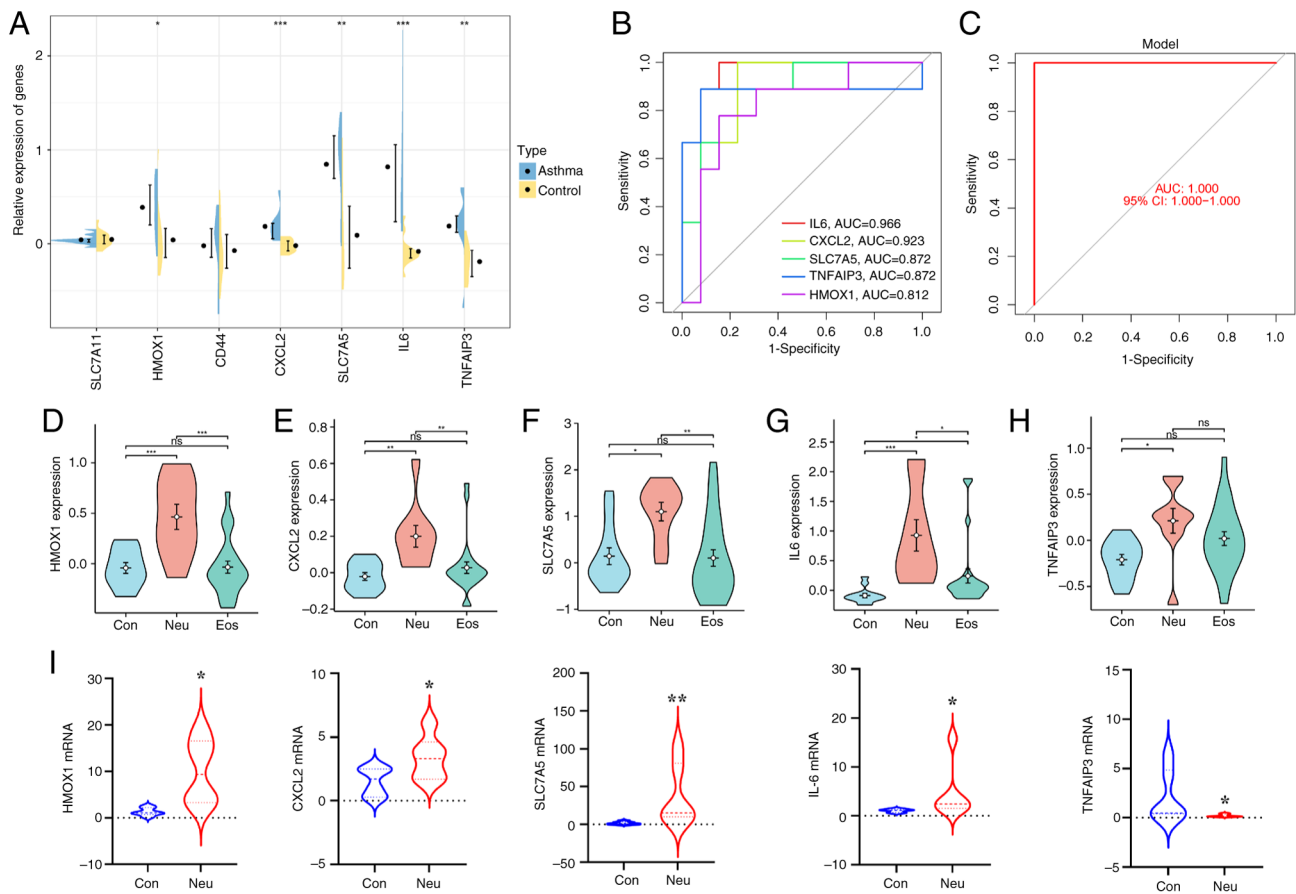
Figure 7. External verification of key DE-FRGs. (A) Comparison of the relative expression levels of hub DE-FRGs of Neu compared with Con groups; the significance level was P<0.05 ; (B and C) ROC curves of the key DE-FRGs. (D-H) Differences in the expression of key DE-FRGs in neutrophilic asthma and eosinophilic asthma from dataset GSE143303. (I) The mRNA expression levels of hub FRGs within mouse lung tissue. * P<0.05 , ** P<0.01 and *** P<0.001 . DE-FRGs, differentially expressed ferroptosis-related genes; Neu, neutrophilic asthma; Con, Control; ROC, receiver operating characteristic; Eos, eosinophilic asthma; ns, not significant; CI, confidence interval.
