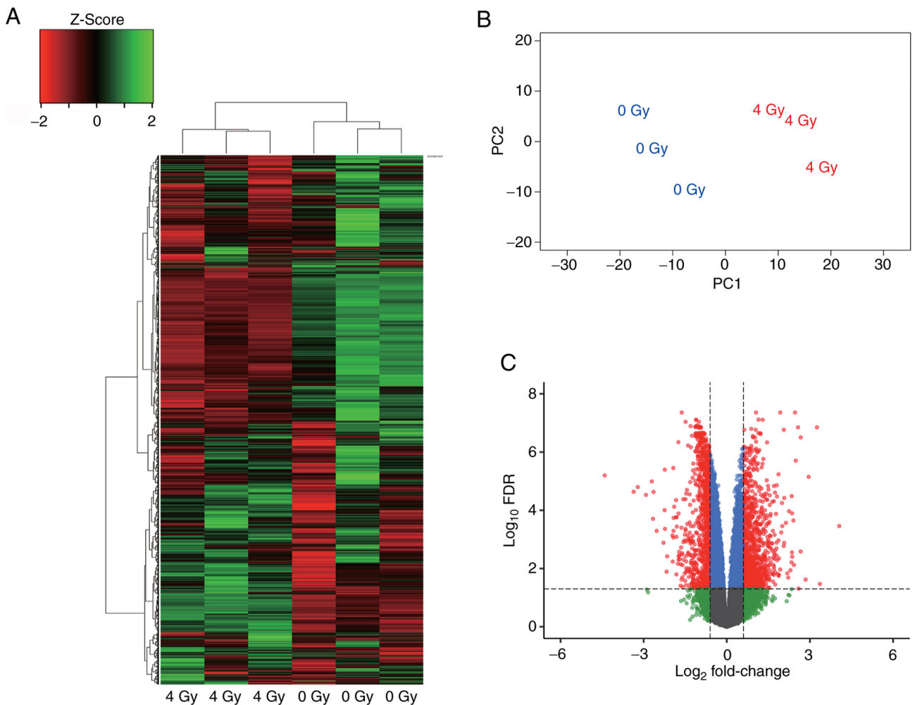
Figure 2. RNA-sequencing reanalysis of HUVECs irradiated with 4 Gy. To examine gene expression in 4 Gy-irradiated and senescence-induced HUVECs, the RNA-sequencing data from GSE130727 (SRR9016151 to SRR9016156) were reanalyzed. (A) Heat map showing hierarchical clustering of the gene expression profiles of 4 Gy-irradiated HUVECs (4 Gy) and nonirradiated HUVECs (0 Gy). Each row represents a gene and each column represents a sample. Gene expression levels were normalized, with green indicating upregulation and red indicating downregulation. (B) PCA plot showing the distribution of 4 Gy-irradiated (red) and nonirradiated (blue) HUVECs. PC1 and PC2 accounted for 79.92 and 14.27% of the total variance, respectively. Each point represents an individual sample. (C) Volcano plot of the differentially expressed genes in 4 Gy-irradiated and nonirradiated HUVECs. Genes with a FDR <0.05 and a fold-change \geq 1.5 are plotted in red. FDR, false discovery rate; PC, principal component; PCA, principal component analysis.
