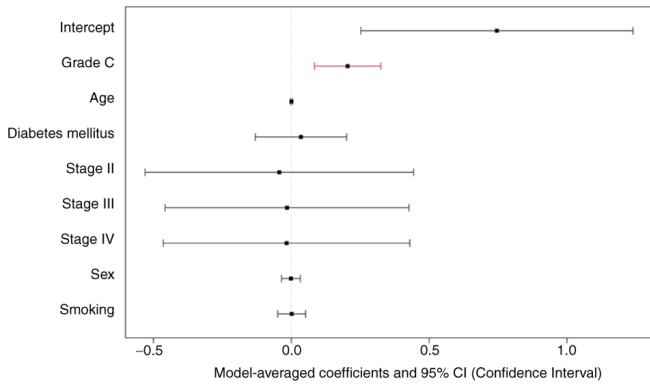
Figure 2. A forest plot was generated to illustrate the relationship between various variables and PD reduction, based on model-averaged coefficient estimates. This analysis was conducted by fitting all subsets of the full model, which included all covariates, and averaging the best-supported models (those with a difference in AIC from the best-supported model of < 2 ). The dredge and model.avg functions from the MuMIn R package were used. PD, probing depth; AIC, Akaike Information Criterion.
