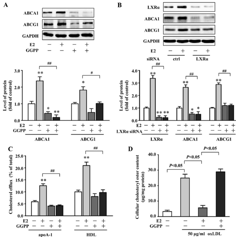
Figure 4. Role of LXR \alpha in E2 activity in vascular smooth muscle cells (VSMCs). (A) VSMCs were pretreated with geranylgeranyl pyrophosphate (GGPP) (20 \mu M) for 2 h, and then treated with E2 (10 nM) for 24 h. The protein expression of ATP-binding cassette transporters ABCA1 and ABCG1 was determined by western blot analysis. (B) VSMCs were transfected with either control or LXR \alpha siRNA (100 nM) for 24 h, followed by E2 (10 nM) for an additional 24 h. LXR \alpha , ABCA1 and ABCG1 protein expression was determined by western blot analysis. (C and D) Prior to treatment with E2 (10 nM), VSMCs were treated with GGPP for 2 h. Cholesterol efflux and intracellular cholesteryl ester content were assessed. The data represent the mean \pm standard error of the mean (SEM). * P <0.05 and ** P <0.01 vs. the control group; # P <0.05 and ## P <0.01 vs. the E2-treated alone group. Each experiment was performed three or four times. E2, 17 \beta -estradiol.
