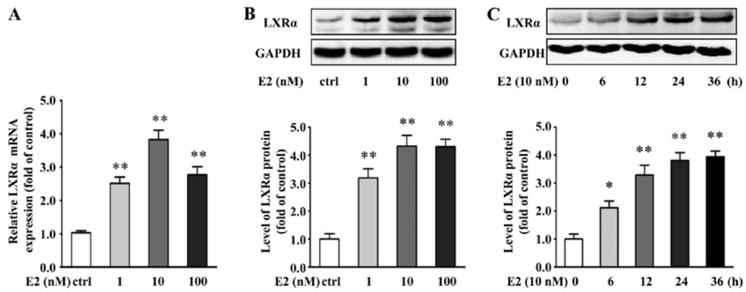
Figure 3. Effects of E2 on LXR \alpha expression in vascular smooth muscle cells (VSMCs). (A and B) VSMCs were incubated with different concentrations of E2 for 24 h. The mRNA and protein expression of LXR \alpha was determined by real-time polymerase chain reaction (PCR) and western blot analysis, respectively. (C) VSMCs were treated with E2 (10 nM) for different time periods. The protein levels of LXR \alpha were determined by western blot analysis. The data represent the mean \pm standard error of the mean (SEM). * P <0.05 and ** P <0.01 vs. control group. Each experiment was performed three times. E2, 17 \beta -estradiol.
