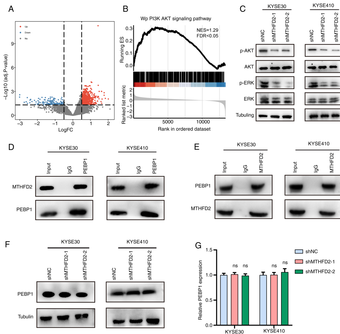
Figure 5. MTHFD2 interacts with PEBP1 and promotes AKT and ERK signaling pathway activation in esophageal squamous cell carcinoma. (A) Differentially expressed genes between patients with high and low MTHFD2 expression. (B) Gene Set Enrichment Analysis indicating enrichment of the PI3K/AKT signaling pathway in the high-MTHFD2 group. (C) Western blot analysis following MTHFD2 knockdown in KYSE30 and KYSE410 cells. Co-immunoprecipitation assay detecting the interaction between MTHFD2 and PEBP1. Immunoprecipitates were probed with (D) anti-MTHFD2 and (E) anti-PEBP1. (F) Western blot and (G) quantitative PCR showing protein and mRNA levels of PEBP1 following MTHFD2 knockdown. ns, not significant; NES, normalized enrichment score; FDR, false discovery rate; MTHFD2, methylenetetrahydrofolate dehydrogenase 2; PEBP1, phosphatidylethanolamine-binding protein 1; sh, short hairpin; NC, negative control; adj.p-value, adjusted P-value; FC, fold-change.
