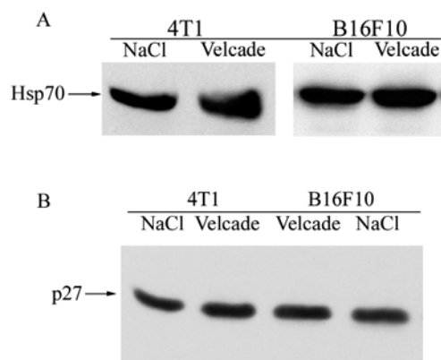
Figure 5. Western blot analysis of Hsp70 and p27. (A) To determine the level of Hsp70 after treatment with Velcade ( 10 \mu\text{M} for 6 h), 30 \mu\text{g} total cellular protein was separated on 10% SDS-PAGE followed by Western blotting with mouse anti-Hsp70 antibody. (B) 25 \mu\text{g} protein was separated on 12% SDS-PAGE followed by Western blotting with mouse monoclonal anti-p27 antibody. The results are representative of two independent experiments.
