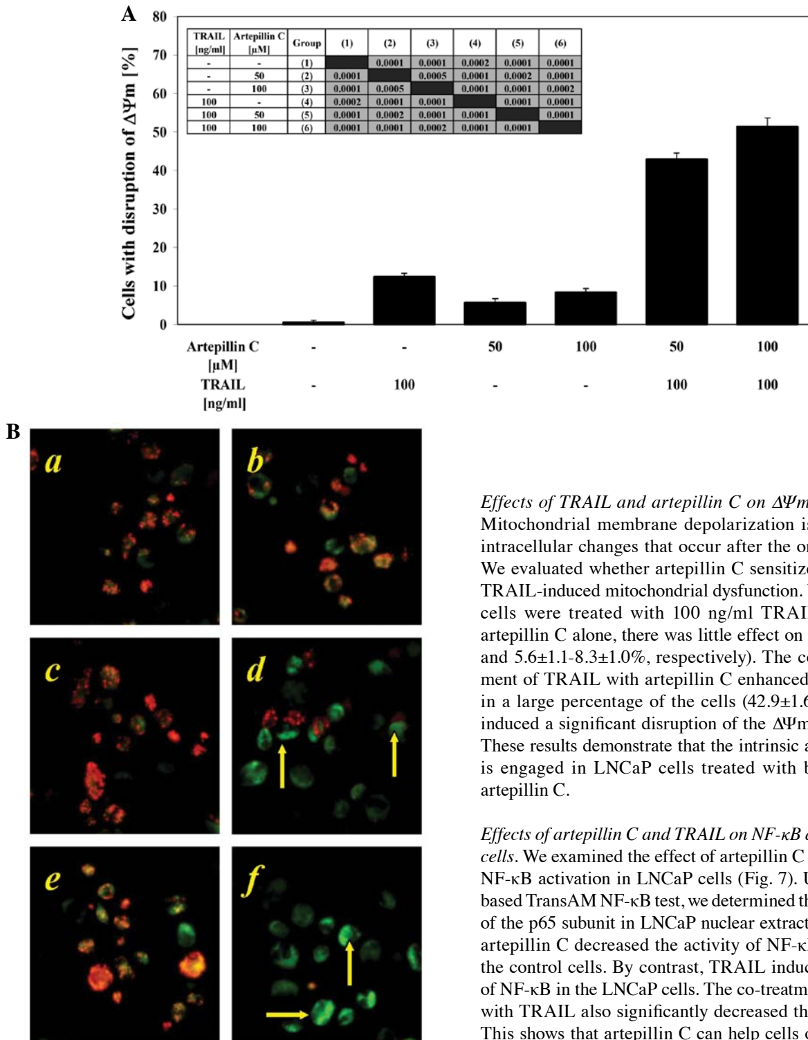
Figure 6. Effects of TRAIL in combination with artepillin C on the mitochondrial membrane potential ( \Delta\Psi_m ) in LNCaP prostate cancer cells. Cells were incubated for 24 h with 100 ng/ml TRAIL and/or 50-100 \mu M artepillin C. The values represent the mean \pm SD of three independent experiments performed in duplicate, n=6 ( p<0.001 TRAIL + artepillin C compared to TRAIL or artepillin C alone as shown by ANOVA). (A) TRAIL in combination with artepillin C induced a loss of \Delta\Psi_m in LNCaP cells. (B) Disruption of \Delta\Psi_m in LNCaP cells was assessed by fluorescent microscopic analysis of DePsiher staining using the following treatment conditions: (a) control cells, (b) cells incubated with 100 ng/ml TRAIL, (c) cells incubated with 50 \mu M artepillin C, (d) cells incubated with 100 ng/ml TRAIL and 50 \mu M artepillin C, (e) incubated with 100 \mu M artepillin C and (f) cells incubated with 100 ng/ml TRAIL and 100 \mu M artepillin C. Red fluorescence is emitted from aggregates of DePsiher, which are formed within the mitochondria of healthy cells. Green fluorescence reveals the monomeric form of the DePsiher molecule, which appears in the cytosol after mitochondrial membrane depolarisation (indicated by arrows).
