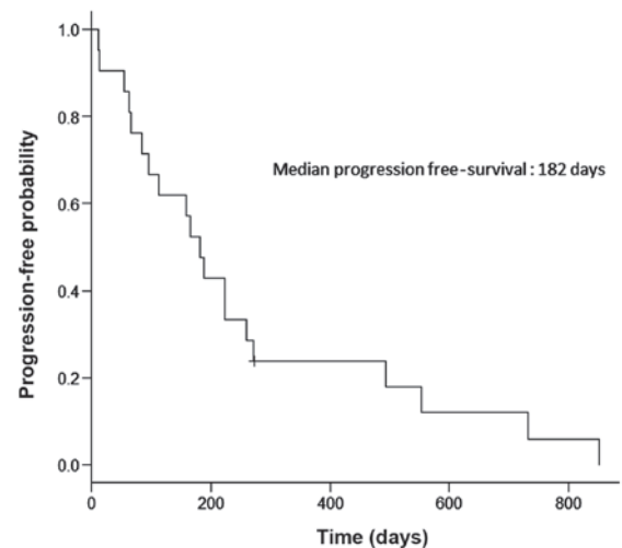
Figure 1. Kaplan-Meier curve for progression-free survival in the 21 patients treated with epidermal growth factor receptor-tyrosine kinase inhibitors. Median progression-free survival, 182 days.
