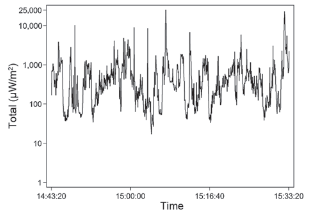
Figure 5. Stockholm Royal Castle. Total radiofrequency field exposure (mean exposure, 721.2 \mu\text{W}/\text{m}^2 , logarithmic scale) over time of one typical exposure round (13 April, 2016; time, 14:43:22-15:33:26).
