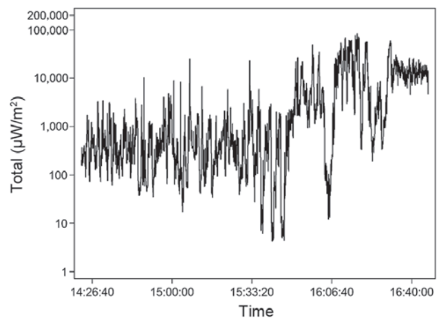
Figure 3. Stockholm Old Town. Total radiofrequency field exposure (mean exposure, 5,371.4 \mu\text{W}/\text{m}^2 , logarithmic scale) over time of one typical exposure round (13 April, 2016; time, 14:22:14-16:46:58).
