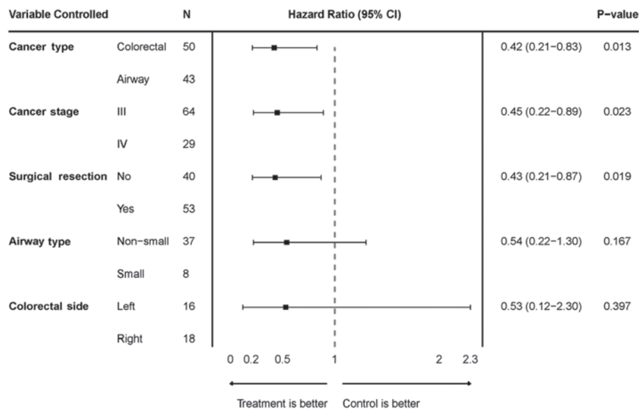
Figure 1. Hazard-ratio plot with 95% CI comparing treatment vs. control in a multivariate analysis controlling for cancer type, cancer stage, surgical resection history, airway cancer type, and colorectal cancer laterality. CI, confidence interval.
