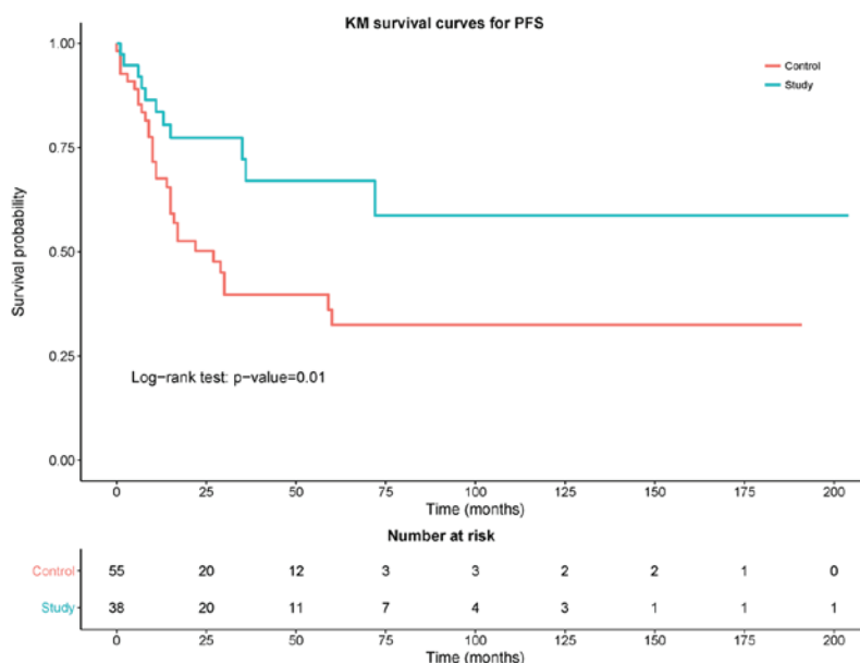
Figure 2. Kaplan-Meier curves of progression-free survival (PFS) of control (red) vs. study (blue) group with number of patients at different time points.
