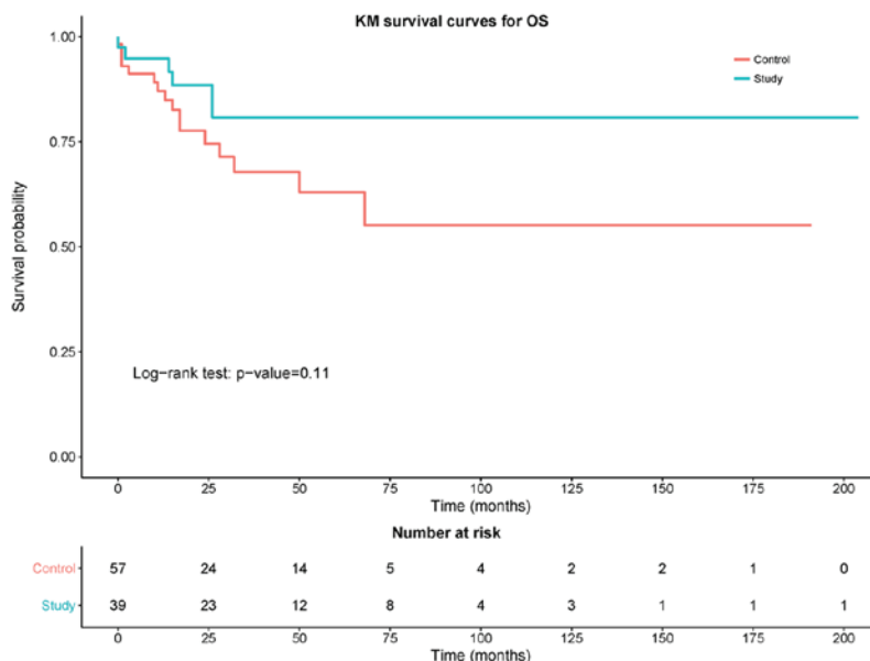
Figure 3. Kaplan-Meier curves of overall survival (OS) of control (red) vs. study (blue) group with number of patients at different time points.
