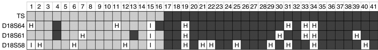
Figure 5. LOH status of the TS locus and of 18q in 41 randomly selected tumor samples. White squares indicate that the LOH status could not be determined either due to microsatellite instability (I) or homozygosity (H). Light grey squares indicate no LOH and dark grey squares indicate LOH. LOH, loss of heterozygosity; TS, thymidylate synthase gene.
