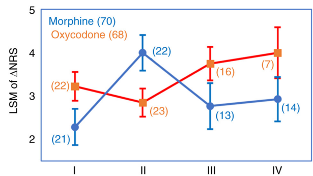
Figure 4. Significance of the \Delta NRS in patients treated with morphine (blue) or oxycodone (orange) is expressed by the LSMs \pm standard error separately for the genotype combinations (rs4778889/rs17809012) of: i) TT/AA; ii) TT/(AG/GG); iii) (TC/CC)/AA; and iv) (TC/CC)/(AG/GG). \Delta NRS, difference in the score on the numerical rating scale for pain recorded prior to the start of opioid treatment and after opioid titration; Numbers in parentheses indicate the numbers of patients. LSMs, least square means; NRS, numerical rating scale.
