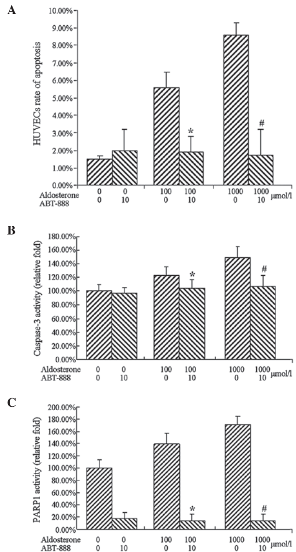
Figure 7. Analysis of (A) apoptotic cells detected by flow cytometry via scattered light changes following treatment with ABT-888-aldosterone. Analysis of (B) caspase-3 activity and (C) PARP1 activity following treatment with ABT-888-aldosterone. * P<0.05 vs. 100 \mu\text{mol/l} aldosterone group, # P<0.05 vs. 1,000 \mu\text{mol/l} aldosterone group. HUVECs, human umbilical vein endothelial cells; PARP, poly (ADP-ribose) polymerase.
