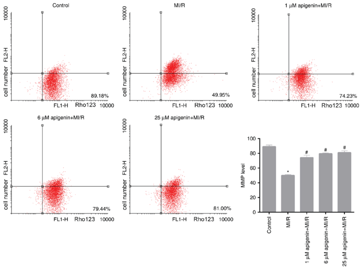
Figure 4. Apigenin modulates the MMP level in MI/R-induced H9C2 cells. Flow cytometry was performed to assess the MMP level in H9C2 cells treated with MI/R, and 1, 6 and 25 \mu M apigenin + MI/R. *P<0.05 vs. control; #P<0.05 vs. MI/R. MMP, mitochondrial membrane potential; MI/R, myocardial ischemia-reperfusion; Rho123, Rhodamine-123.
