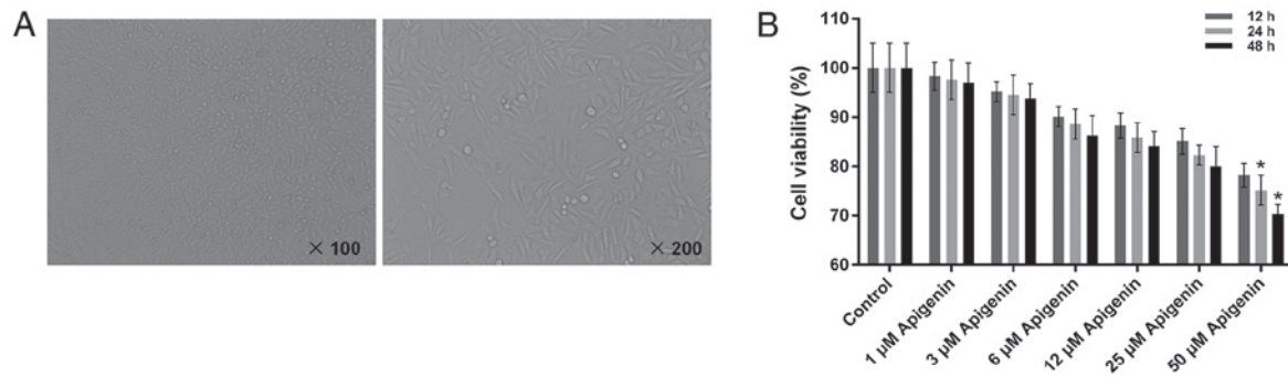
Figure 1. Growth characteristics and cell viability of H9C2 cells treated with apigenin. (A) H9C2 cells were observed with an inverted microscope. (B) A cell counting kit-8 assay was performed to assess the cell viability of H9C2 cells treated with different concentrations of apigenin. * P < 0.05 vs. control.
