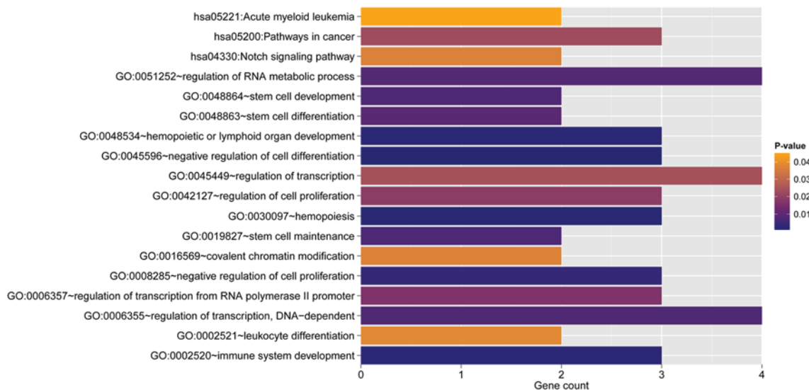
Figure 6. Functional enrichment analysis for co-mutations of Fms related tyrosine kinase 3-Notch 2, DNA methyltransferase 3 \alpha -CCAAT enhancer binding protein \alpha and SET binding protein 1-cyclic adenosine 5'-phosphate response element-binding protein binding protein. GO, gene ontology.
