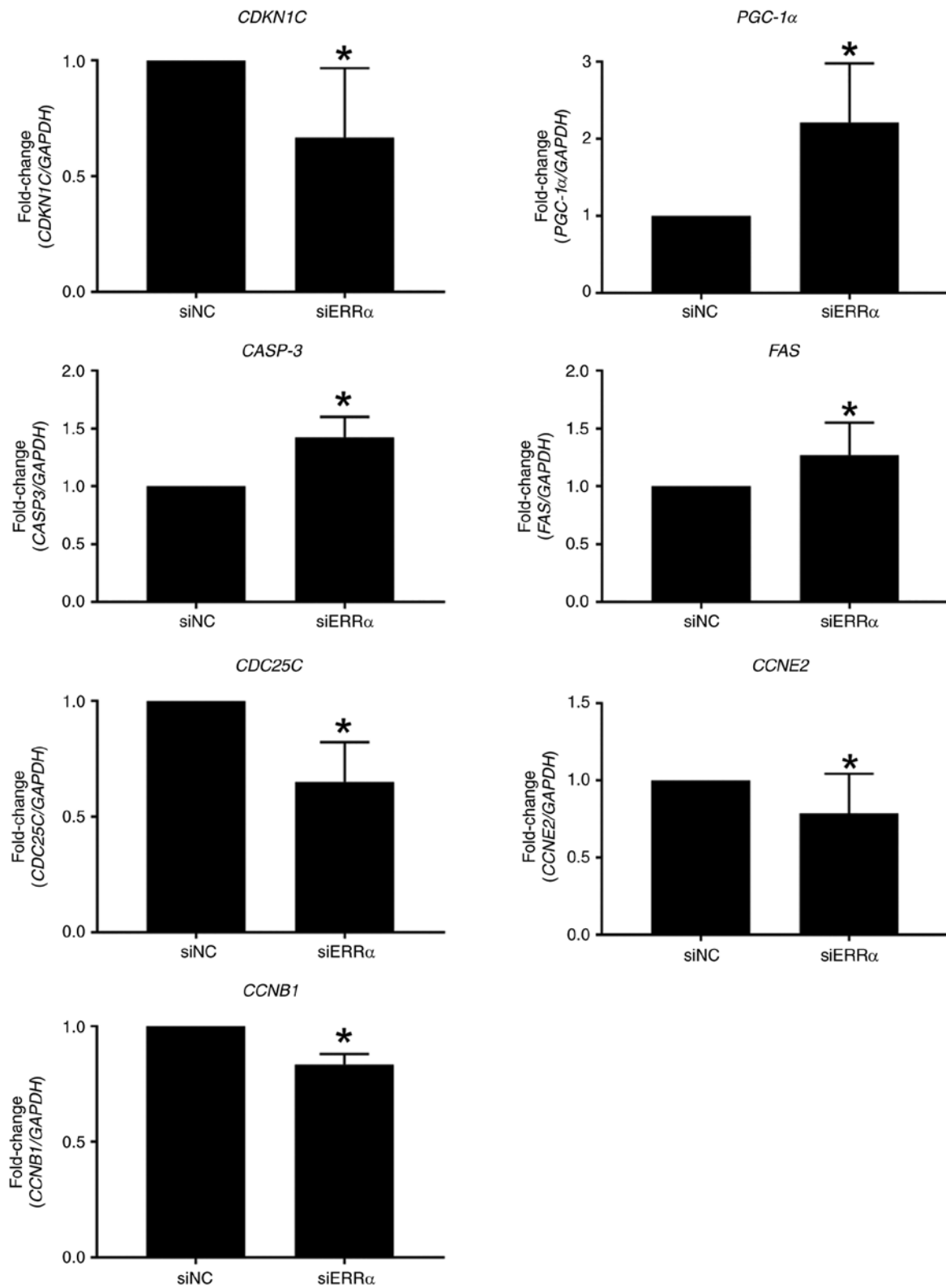
Figure 3. Validation of gene expression in TIG113 cells. TIG113 cells were transfected with siERR \alpha or siNC and cultured for 48 h. The mRNA levels of each gene were quantified using reverse transcription-quantitative PCR. Relative expression was normalized to that of GAPDH . Data represent the mean \pm standard deviation of three independent experiments. *P<0.05 vs. siNC. ERR \alpha , estrogen-related receptor \alpha ; si, small interfering; NC, negative control; CDKN1C , cyclin-dependent kinase inhibitor 1C; PGC-1 \alpha , peroxisome proliferator-activated receptor gamma, coactivator 1 \alpha ; CASP3 , caspase 3; FAS , Fas cell surface death receptor; CDC25C , cell division cycle 25C; CCNE2 , cyclin E2; CCNB1 , cyclin B1.
