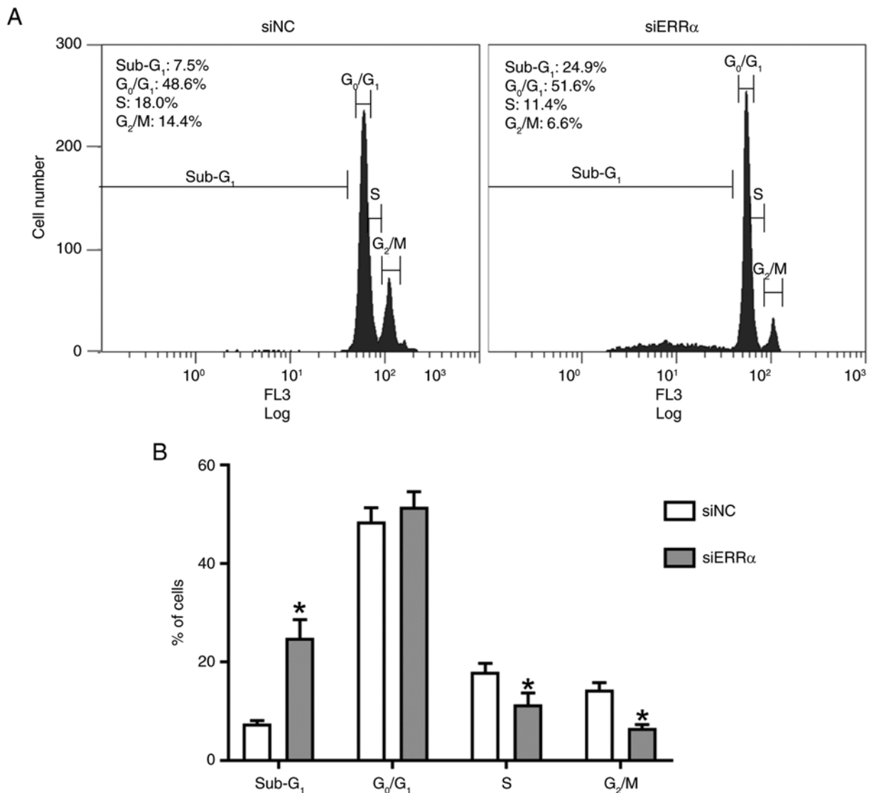
Figure 5. Effect of ERRα silencing on the cell cycle in TIG113 cells. Cell cycle analysis in TIG113 cells treated with siERRα or siNC for 72 h prior to DNA staining and fluorescence-activated cell sorting. (A) Cell cycle plots. (B) Percentages of cells in the Sub-G 1 , G 0 /G 1 , S and G 2 /M phases. Data were analyzed using the MultiCycle AV software and represent the mean ± standard deviation of the mean of three independent experiments. *P<0.05 vs. siNC. ERRα , estrogen-related receptor α; si, small interfering; NC, negative control.
