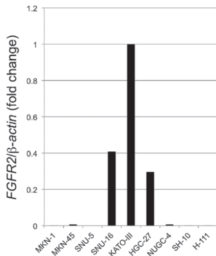
Figure 6. Relative mRNA expression levels of FGFR2 in gastric cancer cell lines, as compared with that of the KATO-III cell line, which was set to an expression level of 1.
