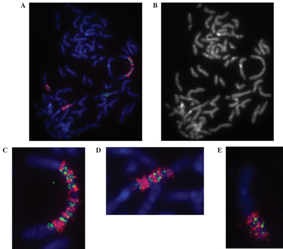
Figure 5. DC-FISH analysis using a probe set consisting of two long-distance polymerase chain reaction products (~10 kb in size). (A) DC-FISH analysis was performed using L4 (red), containing exons 2-5 of APIP , and L1 (green), containing exon 10 of FGFR2 (magnification, x1,000). (B) DAPI image corresponding to the metaphase of (A), which was captured in conjunction with spectral classifications as inverted Q-bands by fluorescence using Hoechst 33258 for the identification of chromosomal breakpoints. (C-E) Enlarged views of tandemly repeated amplifications of APIP and FGFR2 in three homogeneously staining regions within (C). DC-FISH, dual color-fluorescence in situ hybridization.
