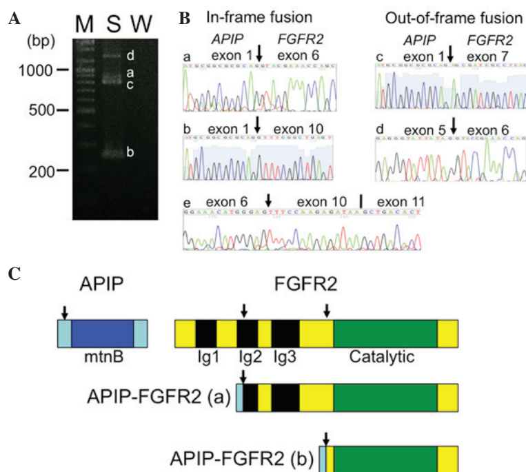
Figure 2. Cloning of the APIP-FGFR2 fusion gene. (A) Detection of APIP-FGFR2 chimeric transcripts using reverse transcription-polymerase chain reaction. Primers were APIP-1-2S and FGFR2-2A. (B) Sequencing of three in-frame (a, b and e) and two out-of-frame (c and d) APIP-FGFR2 fusion transcripts. Vertical arrows indicate the fusion points. Transcripts a, b, c and d correspond to those in (A), while transcript e was not found. (C) Schematic representation of putative APIP, FGFR2 and APIP-FGFR2 proteins. Vertical arrows indicate breakpoints or fusion points. M, size marker; S, SNU-16 cells; W, water; mtnB, methylthioribulose-1-phosphate dehydratase domain; Ig1-3, immunoglobulin-like domain 1-3.
