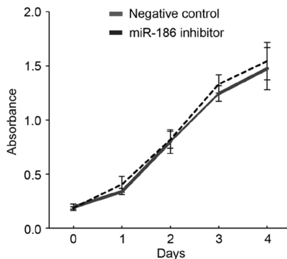
Figure 3. Inhibition of miR-186 did not affect GIST-T1 cellular proliferation. Growth curves are presented for GIST-T1 cells transfected with a miR-186 inhibitor or a negative control generated using cell viability assays. miR, microRNA; GIST, gastrointestinal stromal tumor.
