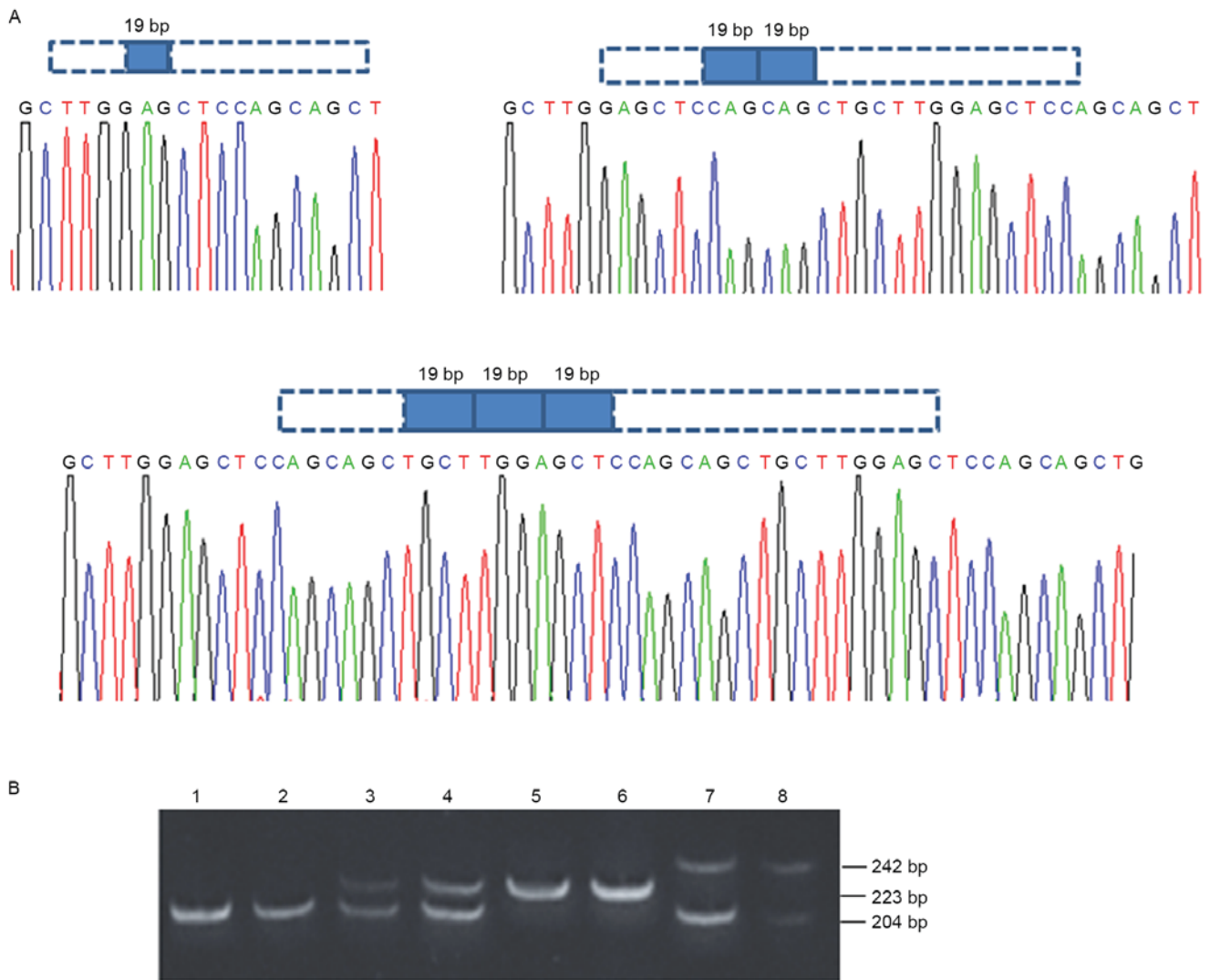
Figure 1. Schematic diagram showing LAPTM4B alleles. (A) Sequencing chromatograms of LAPTM4B alleles. LAPTM4B *1 contains one copy of the 19 bp sequence. LAPTM4B *2 contains two tandem repeats of the 19 bp sequence, and LAPTM4B *3 contains three tandem repeats of the 19 bp sequence. (B) LAPTM4B polymorphisms as verified by polymerase chain reaction analysis. Lanes 1-2, LAPTM4B *1/1; lanes 3-4, LAPTM4B *1/2; lanes 5-6, LAPTM4B *2/2; lanes 7-8, LAPTM4B *1/3 genotype. LAPTM4B , lysosomal protein transmembrane 4β.
