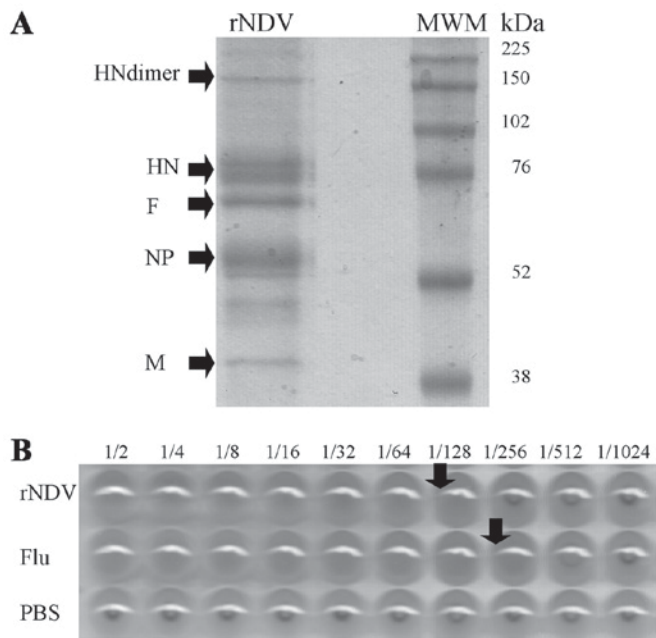
Figure 1. Characterization of proteins and hemagglutinating activity of rNDV. (A) Sodium dodecyl sulfate-polyacrilamide gel from concentrated virus after ultracentrifugation. Arrows indicate molecular weight for the major viral protein: HN as monomer and dimer, F, NP, M. (B) Representative hemagglutination assay for determination of activity and concentration from rNDV-P05 stocks. PBS and Flu vaccine were used as negative and positive controls, respectively. HN, hemagglutinin-neuraminidase; F, fusion protein; NP, nucleocapsid protein; M, matrix protein; MWM, molecular weight marker; kDa, kilo Daltons; rNDV-P05, recombinant attenuated NDV strain P05; PBS, phosphate buffer saline; Flu, polyvalent influenza vaccine.
