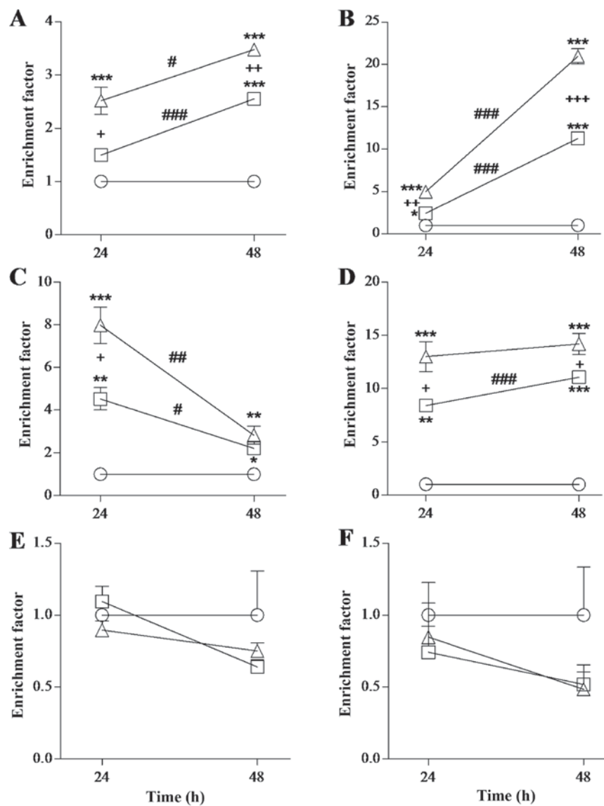
Figure 2. Evaluation of rNDV antitumor activity over different cell lines. (A) HeLa cells, (B) HCC1954 cells, (C) HL-60 cells, (D) HEPG2 cells, (E) A549 cells and (F) PBMC were exposed to different doses of rNDV-P05 [10 (□) and 50 (△) HU] at 24 and 48 h. The EF was evaluated. An equal volume of PBS without virus was added to cells for control assay (○). Results are presented as the mean ± standard error of three independent experiments done for each cell line. *P<0.05, **P<0.01, ***P<0.001 compared to control; +P<0.05, ++P<0.01, +++P<0.001, 10 compared to 50 HU; #P<0.05, ##P<0.01, ###P<0.001, 24 compared to 48 h. All conditions tested on A549 and PBMC were not statistically significant. rNDV-P05, recombinant attenuated NDV strain P05; HeLa, HPV-18 cervix adenocarcinoma; HepG2, hepatoblastoma; HCC1954, breast cancer; HL-60, promyelocytic leukemia; A549, lung carcinoma; PBMC, peripheral blood mononuclear cells; EF, enrichment factor; PBS, phosphate buffer saline; HU, hemagglutination units.
