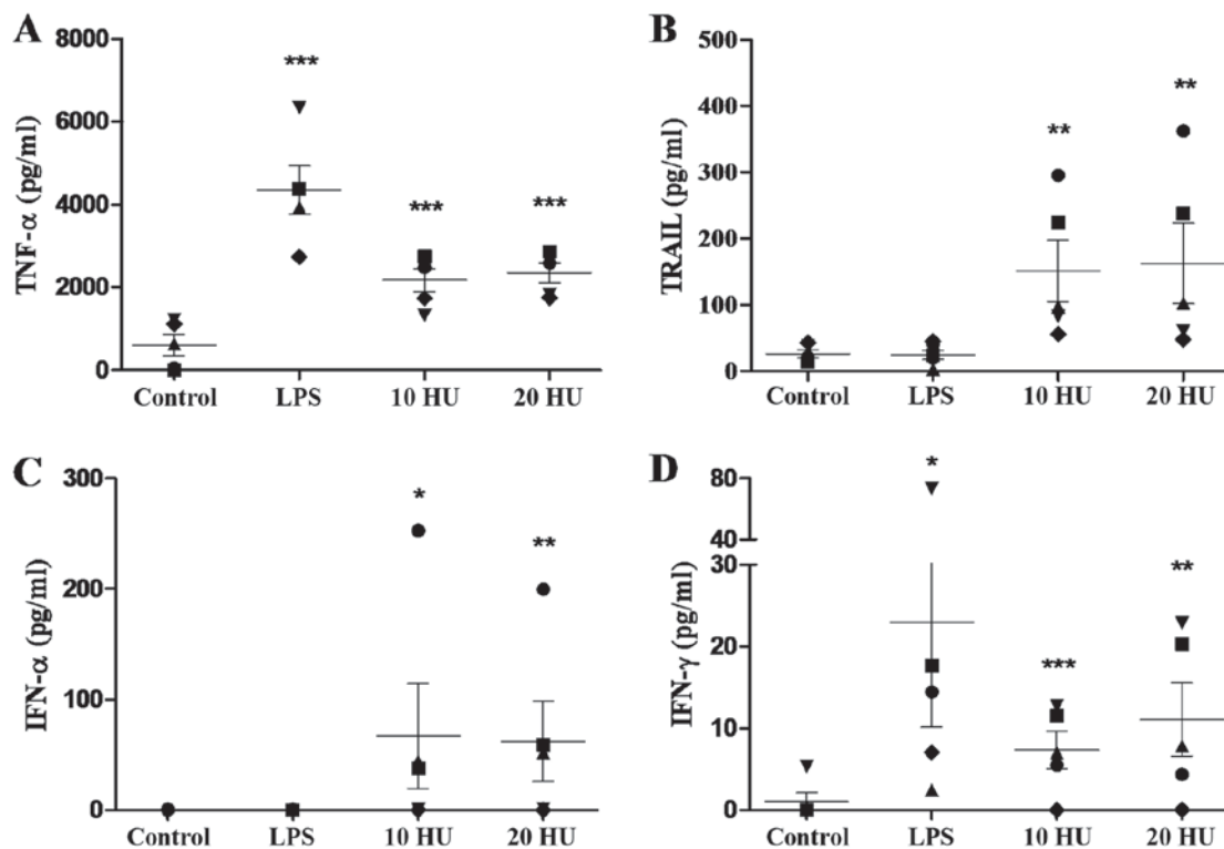
Figure 3. Immunostimulatory activity of rNDV-P05 over PBMC evaluated by ELISA. (A) TNF- \alpha , (B) TRAIL, (C) IFN- \alpha , and (D) IFN- \gamma release by PBMC after 24 h of co-culture with rNDV-P05 (10 and 20 HU/ml) or LPS (5 \mu g/ml). Control cells were incubated with PBS. Results are presented as the mean \pm standard error. Cytokines were determined by duplicate in PBMC isolated from five healthy donors: donor 1 ( \bullet ); 2 ( \blacksquare ); 3 ( \blacktriangle ); 4 ( \blacklozenge ); and 5 ( \blacktriangledown ). * P < 0.05 , ** P < 0.01 , *** P < 0.001 compared to control. rNDV-P05, recombinant attenuated NDV strain P05; PBMC, peripheral blood mononuclear cells; ELISA, enzyme-linked immunosorbent assay; TNF- \alpha , tumor necrosis factor- \alpha ; TRAIL, tumor necrosis factor related apoptosis inducing ligand; IFN, interferon; LPS, lipopolysaccharide; PBS, phosphate buffer saline; HU, hemagglutination units.
