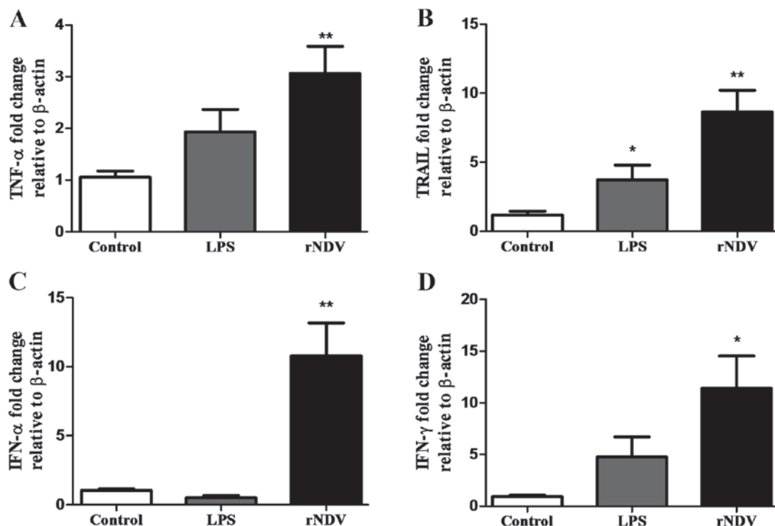
Figure 4. Cytokine expression assessment in PBMC stimulated with rNDV-P05 by quantitative PCR. Changes in the expression of (A) TNF- \alpha , (B) TRAIL, (C) IFN- \alpha , and (D) IFN- \gamma genes were evaluated at 4 h after co-culture with rNDV-P05 20 HU/ml or LPS (5 \mu g/ml). Control cells were incubated with PBS. \beta -actin gene was used as housekeeping gene. Results are presented as the mean \pm standard error. Total RNA from three healthy donors was used and quantified in triplicate. * P < 0.05 , ** P < 0.01 compared to control. PBMC, peripheral blood mononuclear cells; rNDV-P05, recombinant attenuated NDV strain P05; TNF- \alpha , tumor necrosis factor- \alpha ; TRAIL, tumor necrosis factor related apoptosis inducing ligand; IFN, interferon; LPS, lipopolysaccharide; HU, hemagglutination units; PBS, phosphate buffer saline.
