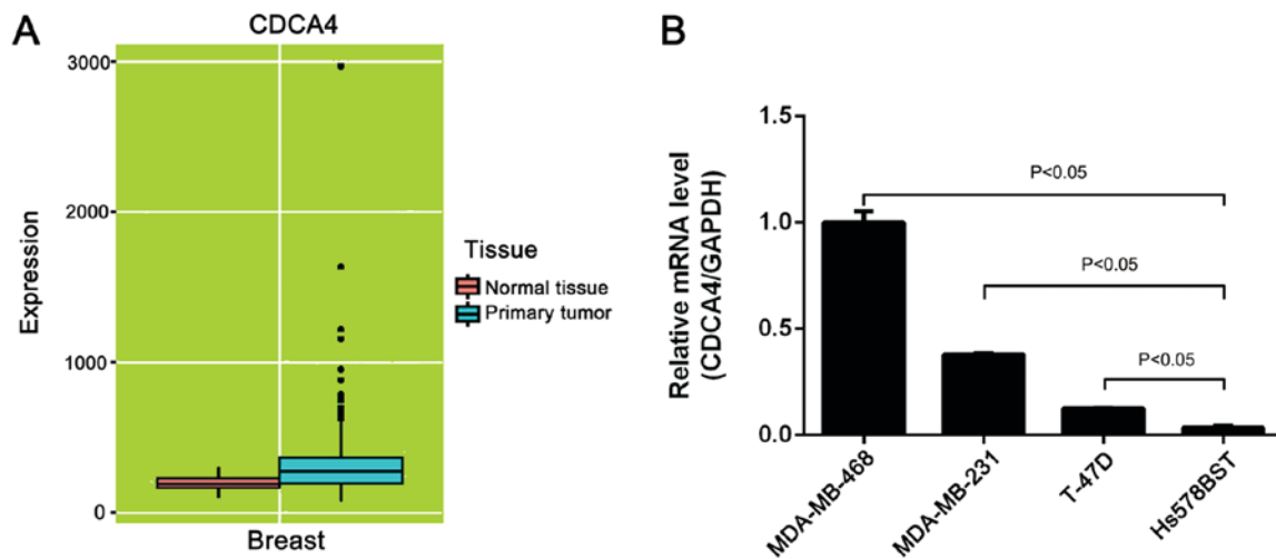
Figure 1. Expression of CDCA4 in breast cancer tissues and cell lines. (A) mRNA expression levels of CDCA4 in normal breast vs. primary breast tumor tissues. CDCA4 expression data were obtained from the online MERAV database ( http://merav.wi.mit.edu ). (B) RT-qPCR. Relative mRNA expression levels of CDCA4 in MDA-MB-231, MDA-MB-468, T-47D and Hs578BST cells were assessed using RT-qPCR. The data were expressed as the means \pm standard deviation. CDCA4, cell division cycle-associated protein 4; RT-qPCR, reverse transcription-quantitative polymerase chain reaction.
