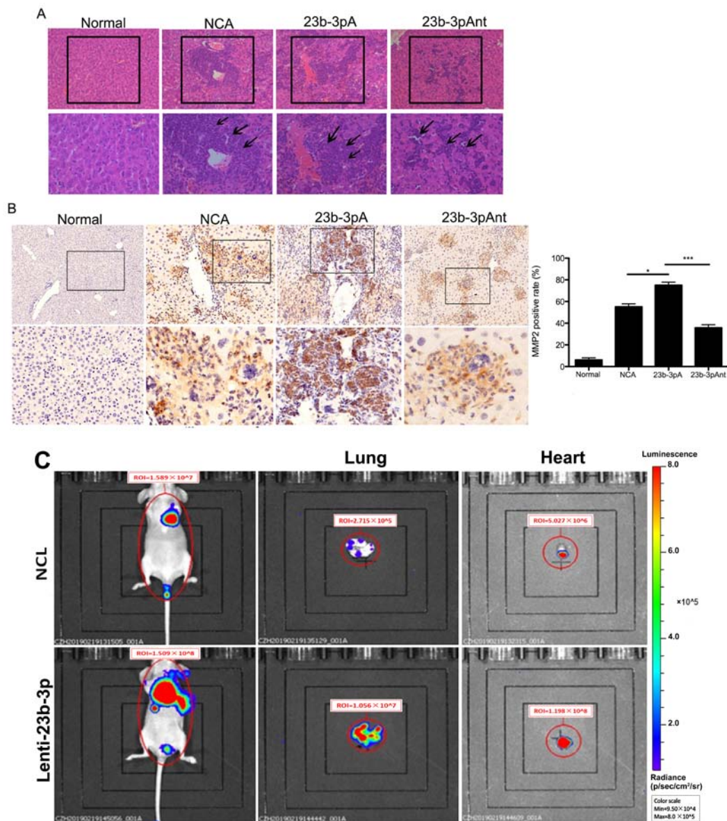
Figure 4. Effect of miR-23b-3p on pancreatic cancer metastasis. (A) At 50 days following creation of the xenograft mouse model, the liver tissues of mice were harvested, and histological analysis was performed to examine the effect of miR-23b-3p on liver metastasis. The images in the upper panel were \times 100 magnified, and images in the lower panel are a magnification of the indicated boxes, at \times 200 magnification. The metastatic lesions were indicated with black boxes and the inflammatory cells were indicated with black arrows. (B) IHC staining of MMP2 in liver tissues. The images in the upper panel were \times 100 magnified, and images in the lower panel are a magnification of the indicated boxes, at \times 200 magnification. The bar graph shows the quantification of IHC staining. * P < 0.05 ; *** P < 0.001 . (C) The BXP-3 cells stably expressing miR-23b-3p were injected into the caudal vein of nude mice, after 52 days, the mice were injected with D-luciferin for 15 min, then the whole-body imaging was acquired using Living Image software. The red circle represents the ROI, and the total luminescence within the ROI was considered as the signal intensity. The mice injected with saline solution only were used as Normal group. 23b-3pAnt, miR-23b-3p antagonist; 23b-3pA, miR-23b-3p agomir; control, negative control agomir; NCL, negative control lentivirus; IHC, immunohistochemical; lenti-23b-3p, miR-23b-3p lentivirus; miR, microRNA; MMP, matrix metalloproteinase; ROI, Region of Interest.
