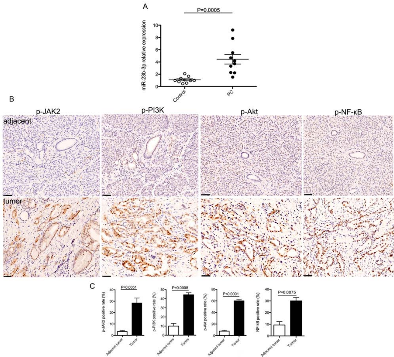
Figure 1. Serum miR-23b-3p levels and tissue expression of p-JAK2, p-PI3K p-Akt and p-NF-κB in patients with PC. (A) Reverse transcription-quantitative PCR was performed to determine the miR-23b-3p levels in the serum of 10 patients with PC and 10 healthy controls. (B) IHC staining was performed to investigate the protein expression level of p-JAK2, p-PI3K p-Akt and p-NF-κB in tumor and adjacent normal tissues using tissue chips. Scale bar, 50 μm. (C) Quantification of IHC staining, indicating the rate of positive staining between the tumor and the control samples (n=40). IHC, immunohistochemical; JAK2, Janus kinase 2; miR, microRNA; PC, pancreatic cancer; p, phosphorylated.
