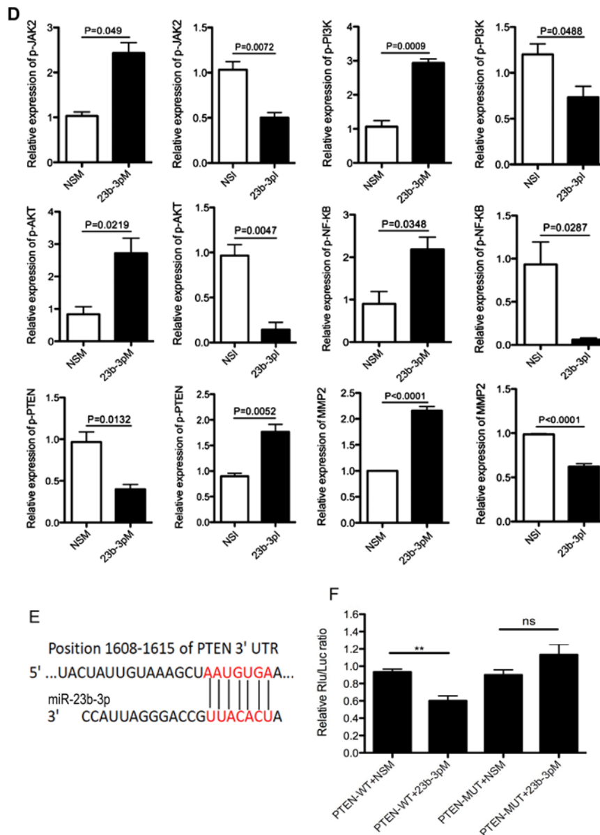
Figure 2. Continued. (D) The bar graphs show the quantification of western blot analysis of the phosphorylated proteins and MMP2. (E) The bioinformatics analysis using TargetScan shows that miR-23b-3p could bind at positions 1,608 to 1,615 of PTEN 3'UTR (the binding sites were indicated as red color). (F) The effect of miR-23b-3p overexpression on the transcriptional activity of the PTEN gene. PANC-1 cells were transfected with 23b-3pM or NSM for 24 h. The luciferase reporter assay was performed to determine the transcriptional activity of the WT PTEN gene and the 3'-UTR-MUT PTEN gene. **P<0.01. 23b-3pI, miR-23b-3p inhibitor; 23b-3pM, miR-23b-3p mimic; IL, interleukin; JAK2, Janus kinase 2; miR, microRNA; MMP, matrix metalloproteinase; MUT, mutated; NS, not significant; NSI, non-specific inhibitor; NSM, non-specific mimic; p-, phosphorylated; RT-qPCR, reverse transcription-quantitative PCR; UTR, untranslated region; WT, wild-type; Rlu, Renilla luciferase.
