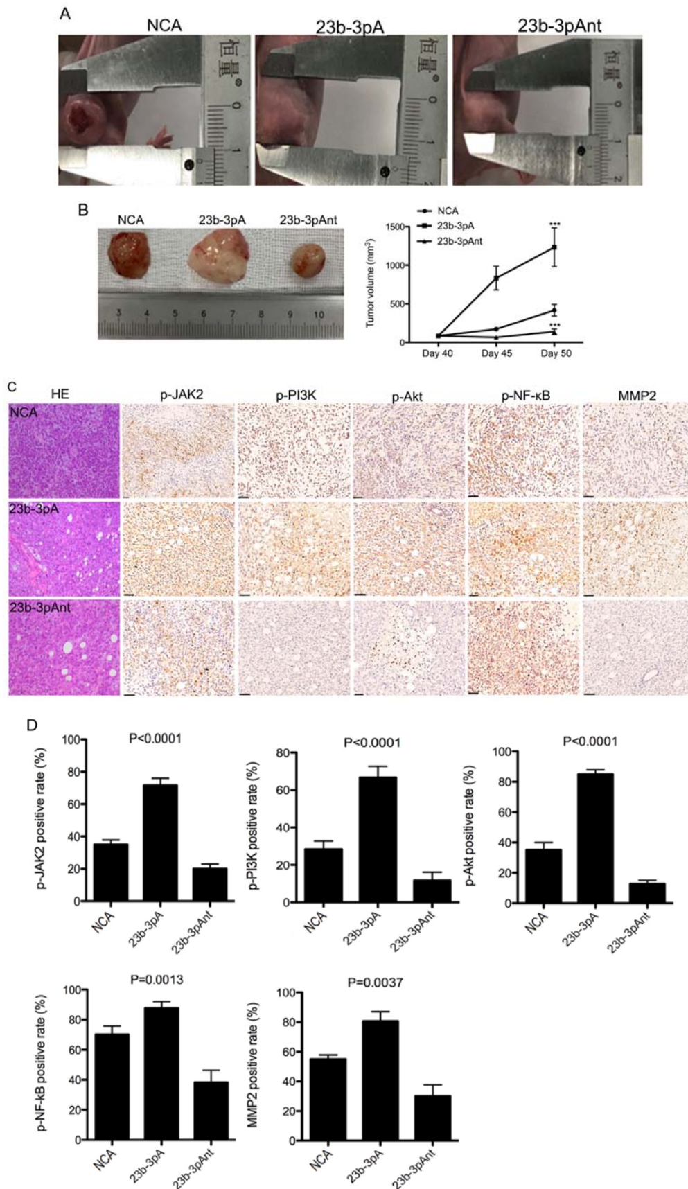
Figure 3. Effect of miR-23b-3p on cell tumorigenesis and JAK/Akt/NF- \kappa B signaling pathway activation in pancreatic cancer. (A) At day 40, 23b-3pA, 23b-3pAnt or NCA was injected into PANC-1 cell-derived subcutaneous tumors in a xenograft mouse model every 3 days. The width and length of tumor were measured and the volume was calculated in vivo every 5 days. (B) At 50 days, subcutaneous tumors were harvested. The tumor volume curve was created. *** P < 0.001 compared with control. (C) Hematoxylin and eosin staining of PANC-1 cell-derived tumors and immunohistochemical staining of p-JAK2, p-PI3K, p-Akt, p-NF- \kappa B and MMP2 in PANC-1 cell-derived tumor sections. Scale bar, 50 \mu m. (D) Quantification of the positive staining rate for p-JAK2, p-PI3K, p-Akt, p-NF- \kappa B and MMP2 expression. 23b-3pAnt, miR-23b-3p antagomir; 23b-3pA, miR-23b-3p agomir; NCA, negative control agomir; JAK2, Janus kinase 2; miR, microRNA; MMP, matrix metalloproteinase.
