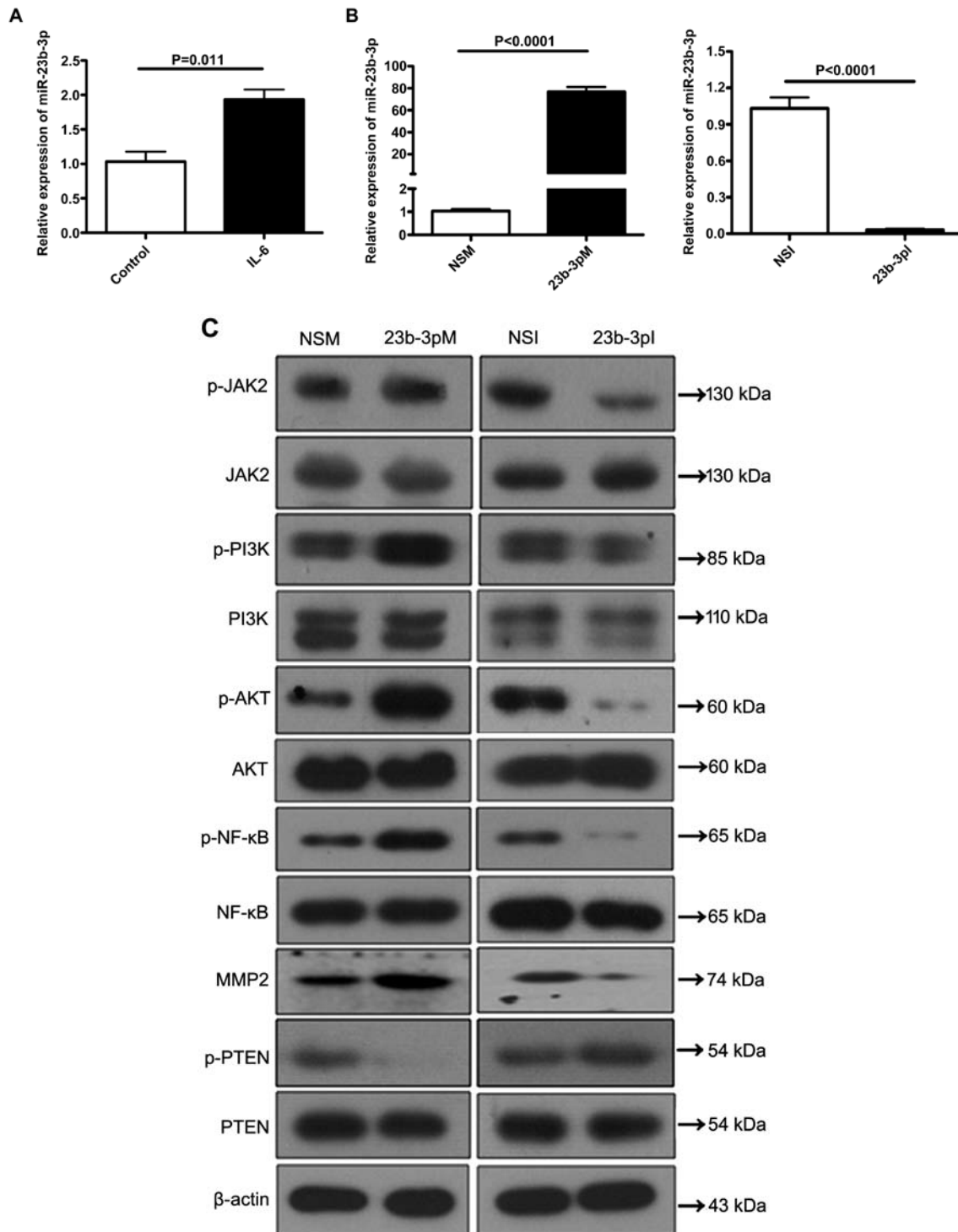
Figure 2. miR-23b-3p regulates the JAK/Akt/NF- \kappa B signaling pathway in pancreatic cancer cells. (A) RT-qPCR was performed to detect the mRNA levels of miR-23b-3p in PANC-1 cells in response to IL-6 stimulation. (B) PANC-1 cells were transfected with 23b-3pM, 23b-3pI and the respective controls, NSM and NSI for 72 h, and the relative expression of miR-23b-3p was measured using RT-qPCR. (C) The effect of miR-23b-3p overexpression and inhibition on the expression levels of proteins in the JAK/Akt/NF- \kappa B signaling pathway. Western blot assays were performed to detect the expression of JAK2, p-JAK2, PI3K, p-PI3K, Akt, p-Akt, NF- \kappa B, p-NF- \kappa B, MMP2, PTEN and p-PTEN. \beta -actin was used as the internal control for total protein, while total protein was used as the internal control for the phosphorylated protein.
