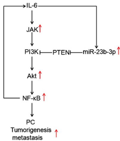
Figure 5. Signaling pathway diagram for PC tumorigenesis and metastasis regulated by miR-23b-3p. The activation role is indicated by the black arrow, while the inhibition role is indicated by the suppression symbol, and the red arrow indicates upregulation. IL-6, interleukin-6; JAK, Janus kinase; miR, microRNA; PC, pancreatic cancer; miR, microRNA.
