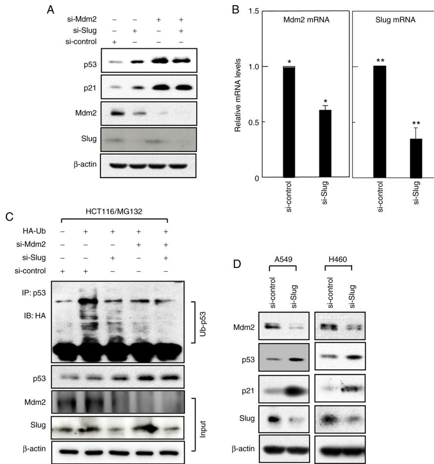
Figure 4. Slug increases Mdm2 expression. (A) HCT116 cells were treated with siRNAs targeting Slug or Mdm2 in the combination indicated. After 24 h of incubation, expression levels of the specified proteins were compared using western blotting. (B) Mdm2 and Slug mRNA levels in HCT116 cells, treated with control or Slug siRNA, were compared by reverse transcription-quantitative PCR. (C) HCT116 cells were transfected with the expression vector for HA-tagged ubiquitin along with siRNAs targeting Slug or Mdm2 in the indicated combinations. The transfectants were treated with MG132 (10 μM) for 2 h. The precipitated proteins were analyzed by western blotting using anti-HA and anti-p53 antibodies. Effects of siRNAs were confirmed by analyzing cell lysates using anti-Mdm2 and anti-Slug antibodies (input). (D) A549 and H460 cells were treated with control or Slug siRNA for 24 h. Levels of the indicated proteins were compared. *P<0.005, si-control vs. si-Slug for Mdm2 mRNA. **P<0.05, si-control vs. si-Slug for Slug mRNA. siRNA, small interfering RNA; Slug, zinc finger protein SNAI2; HA-Ub, HA-ubiquitin; IP, immunoprecipitation; IB, immunoblotting.
