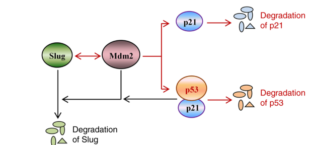
Figure 5. Schematic model representing the functional relationship between Slug, Mdm2, p53 and p21. Slug increased cellular levels of Mdm2 mRNA and protein. As Mdm2 could stabilize Slug mRNA by binding to it, an amplification loop between Slug and Mdm2 expression appeared to exist (indicated by two-headed arrow). Mdm2 could act on p53 and p21, inducing their degradation. While Mdm2 was not required p53 for p21 degradation, its action on p53 required p21 since the p53/p21 interaction promoted the p53/Mdm2 interaction. This oncogenic situation is indicated by red arrows. Mdm2 could also induce proteolytic cleavage of Slug, which was facilitated by the p53/p21 complex. This tumor-suppressing pathway is indicated by black arrows. This model suggested that Mdm2 could exert dual functions by mediating either the tumor-promoting function of Slug or tumor-suppressing function of the p53/p21 complex; the balance between these two opposing pathways may change depending on the external environment and internal physiology of cells. Slug, zinc finger protein SNAI2.
