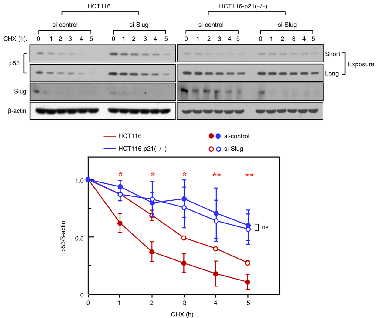
Figure 2. Slug promotes p53 protein degradation in a p21-dependent manner. HCT116 cells and their p21-knockout variants were treated with control or Slug siRNA. After 24 h of recovery, the cells were additionally treated with CHX (10 μM) and further incubated for the indicated periods. p53 levels were analyzed by western blotting and normalized to those of β-actin. Western blotting results are representative of both short and long exposures for more precise comparison. Their mean values and standard deviations are shown in the plots. *P<0.005, **P<0.05 si-control vs. si-Slug in HCT116 cells. ns, non-significant; siRNA, small interfering RNA; Slug, zinc finger protein SNAI2; CHX, cycloheximide.
