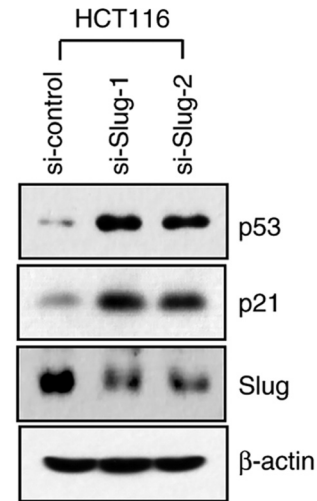
Figure 1. Slug decreases cellular levels of p53 and p21. HCT116 cells were treated either with a control or two sets of Slug-targeting siRNAs. After 24 h of incubation, cellular expression levels of p53, p21 and Slug were compared using western blotting. \beta -actin was used as the loading control. siRNA, small interfering RNA; Slug, zinc finger protein SNAI2.
