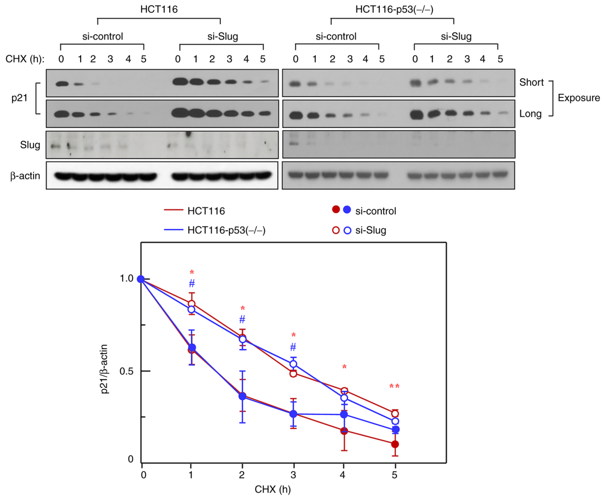
Figure 3. Slug promotes p21 protein degradation in a p53-independent manner. HCT116 cells and their p53-knockout variants were treated with control or Slug siRNA for 24 h, and then incubated in the presence of CHX (10 \mu M) for the indicated periods. p21 and Slug levels were analyzed. * P < 0.005 , ** P < 0.05 si-control vs. si-Slug in HCT116 cells. # P < 0.005 si-control vs. si-Slug in p53-knockout variants. siRNA, small interfering RNA; Slug, zinc finger protein SNAI2; CHX, cycloheximide.
