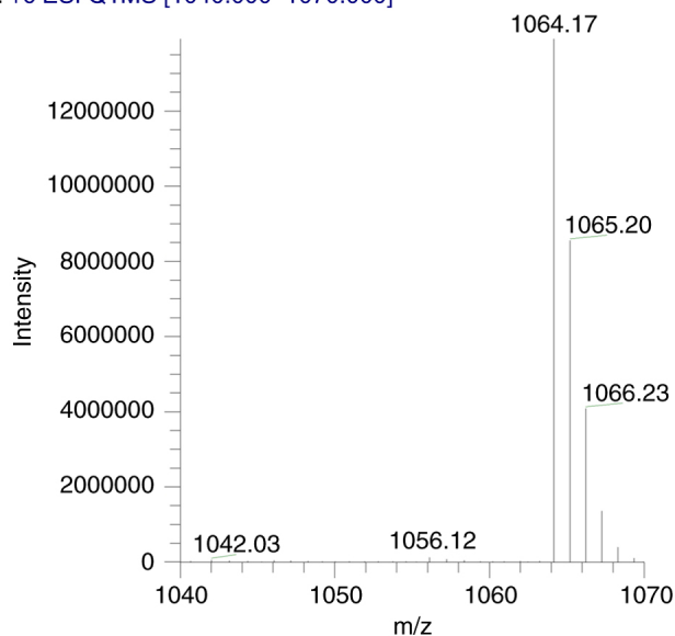
Figure 3. Electrospray ionization mass spectrum (ESI-MS) of IDD-1040. RT, retention time; AV, average; NL, noise level; +c ESI Q1 MS, positive-mode electrospray ionization quadrupole 1 mass spectrometry.
