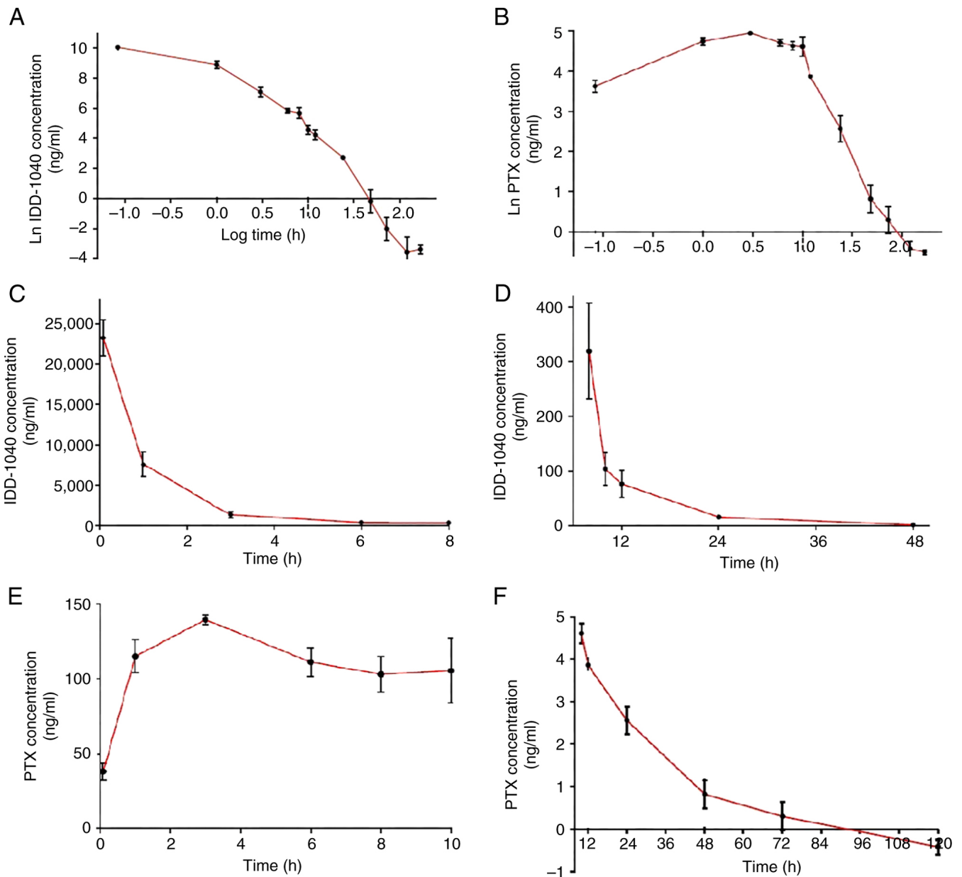
Figure 4. Pharmacokinetic profiles of IDD-1040 and its metabolite PTX. An In-log conversion was applied to facilitate the visualization of all data collectively for (A) IDD-1040 and (B) PTX. Line graphs showing the (C) initial and (D) terminal phases of the pharmacokinetics of IDD-1040, both of which show exponential decay. Pharmacokinetic profiles of PTX at the (E) initial and (F) terminal phases. PTX, paclitaxel; In-log, natural log-common log.
