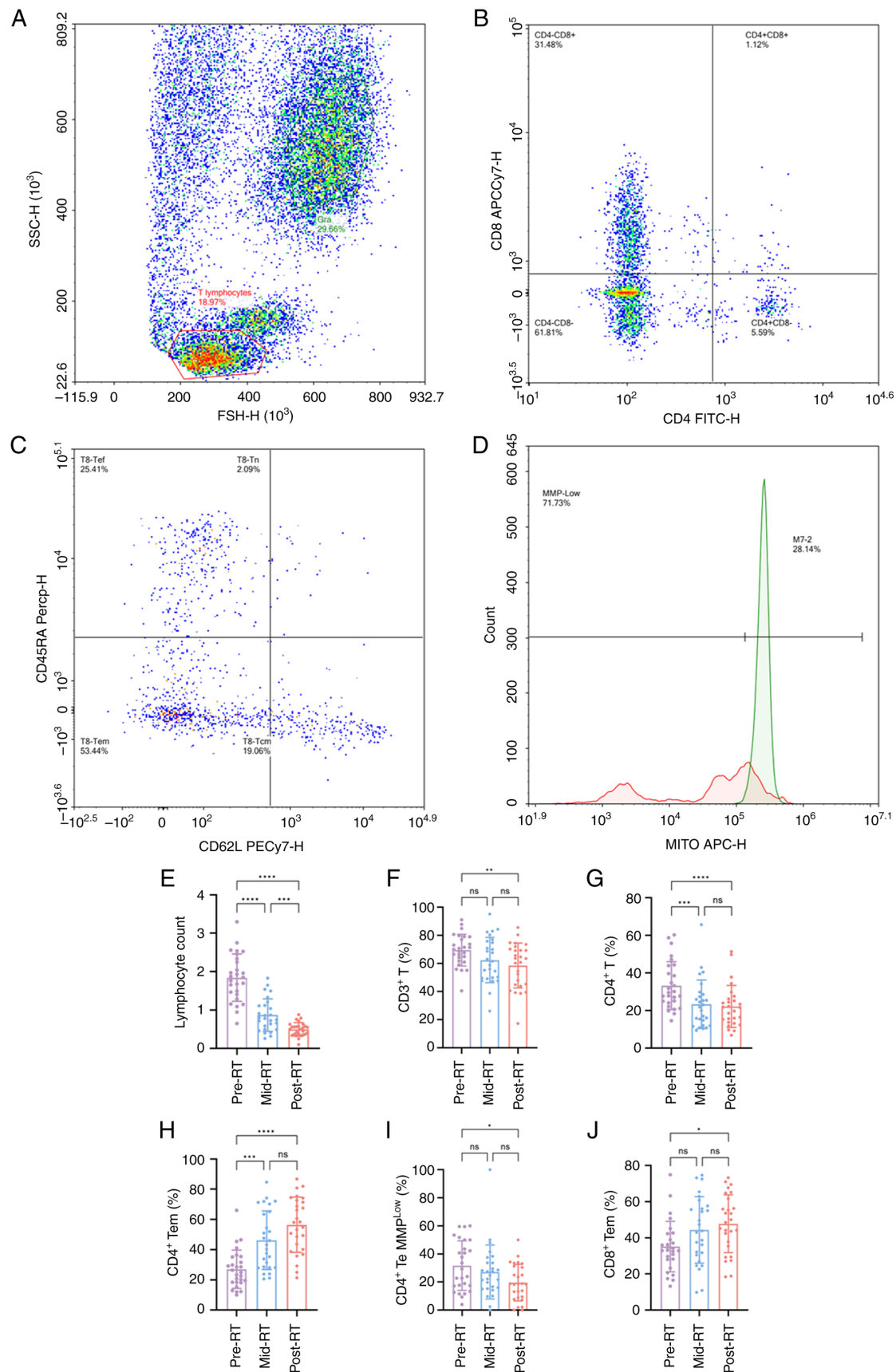
Figure 1. Flow cytometry and changes in immune cells during RT. Gating strategy in flow cytometry. (A) FSC/SSC plot of the lymphocyte populations. (B) CD4/CD8 scatter of the CD4 + CD8 + and CD4 + CD8 - cell populations. (C) CD62L/CD45RA scatter plots of the Tn, Tem, Tef and Tef cell populations. (D) Count/MITO APC-H of the Tem, Tn, Tcm and Tef cell populations, using a dichotomous gate to calculate the percentage of lymphocytes and fluorescence intensity in each population. Changes in the (E) number of lymphocytes, proportion of (F) CD3 + T cells, (G) CD4 + T cells and (H) CD4 + Tem cells, (I) MMP Low in CD4 + Te cells and (J) proportion of CD8 + Tem cells during RT. n=27 per group. *P<0.05; **P<0.01; ***P<0.001; ****P<0.0001. RSC, forward scatter; SSC, side scatter; ns, not significant; RT, radiotherapy; Tem, memory-effector T cells; Te, effector cells T; Tef, effector T cells; Tn, Naïve T cells; Tcm, central memory T cells; MMP, mitochondrial membrane potential.
