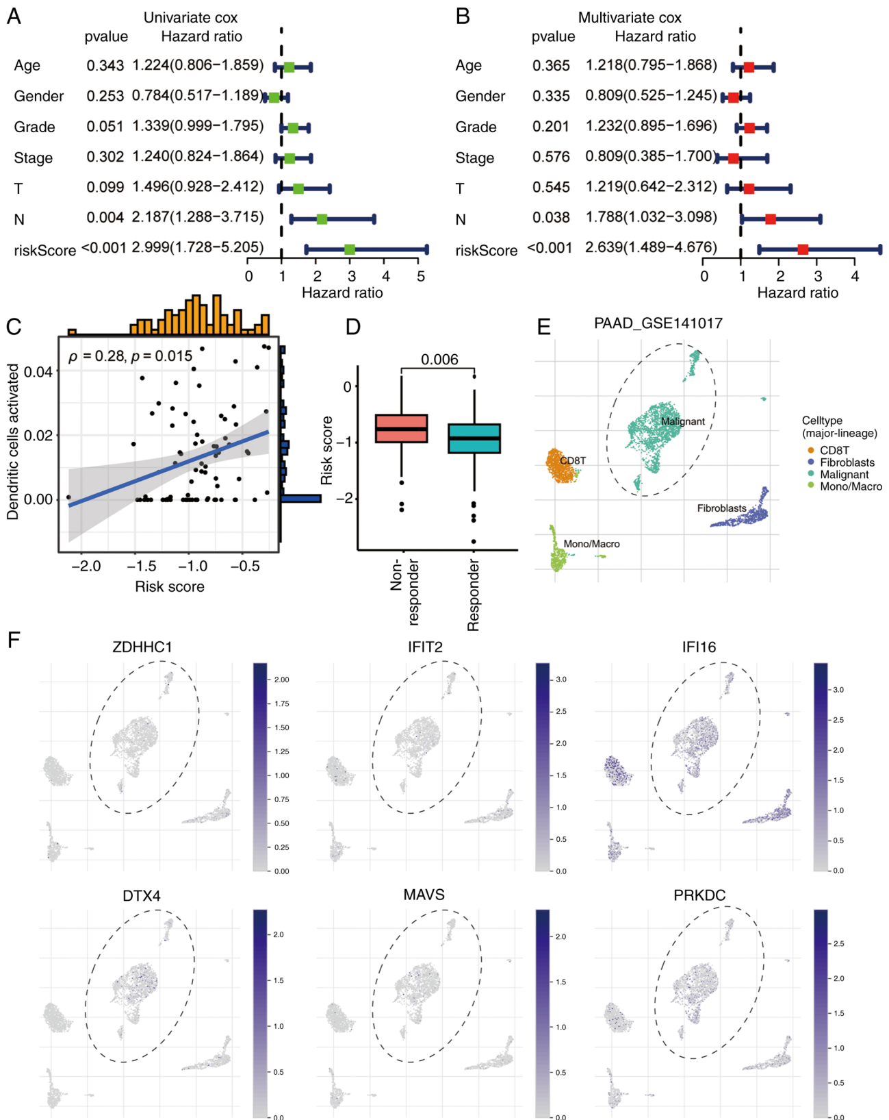
Figure 6. Independent prognostic value and immunotherapy relevance of the STING-related risk signature in PAAD. (A) Univariate Cox regression analysis of clinical parameters and risk score. (B) Multivariate Cox regression confirming the risk score as an independent prognostic factor after adjusting for covariates in (A). (C) Correlation analysis of risk score and activated dendritic cell abundance. 'Dendritic cells activated' represents proportion scores derived from the xCell algorithm (0-1 scale), quantifying relative abundance in the tumor microenvironment. Correlation was assessed using Spearman's rank correlation analysis (Spearman's \rho=0.28 ; P=0.015 ). (D) Higher risk scores in immunotherapy non-responders vs. responders (Mann-Whitney U test). Single-cell RNA sequencing (GSE141017) visualization of STING1 signature gene expression: (E) t-SNE plot showing cell-type distribution. (F) Feature plots of signature gene expression across the PAAD tumor microenvironment. STING, stimulator of interferon genes; PAAD, pancreatic ductal adenocarcinoma; T, tumor; N, node; CD8T, T-cell surface glycoprotein CD8; ZDHHC1, zinc finger DHHC-type containing 1; IFIT2, interferon-induced protein with tetratricopeptide repeats 2; IFI16, interferon \gamma inducible protein 16; DTX4, deltex E3 ubiquitin ligase 4; MAVS, mitochondrial antiviral-signaling protein; PRKDC, protein kinase DNA-activated catalytic subunit; PAAD, pancreatic adenocarcinoma.
