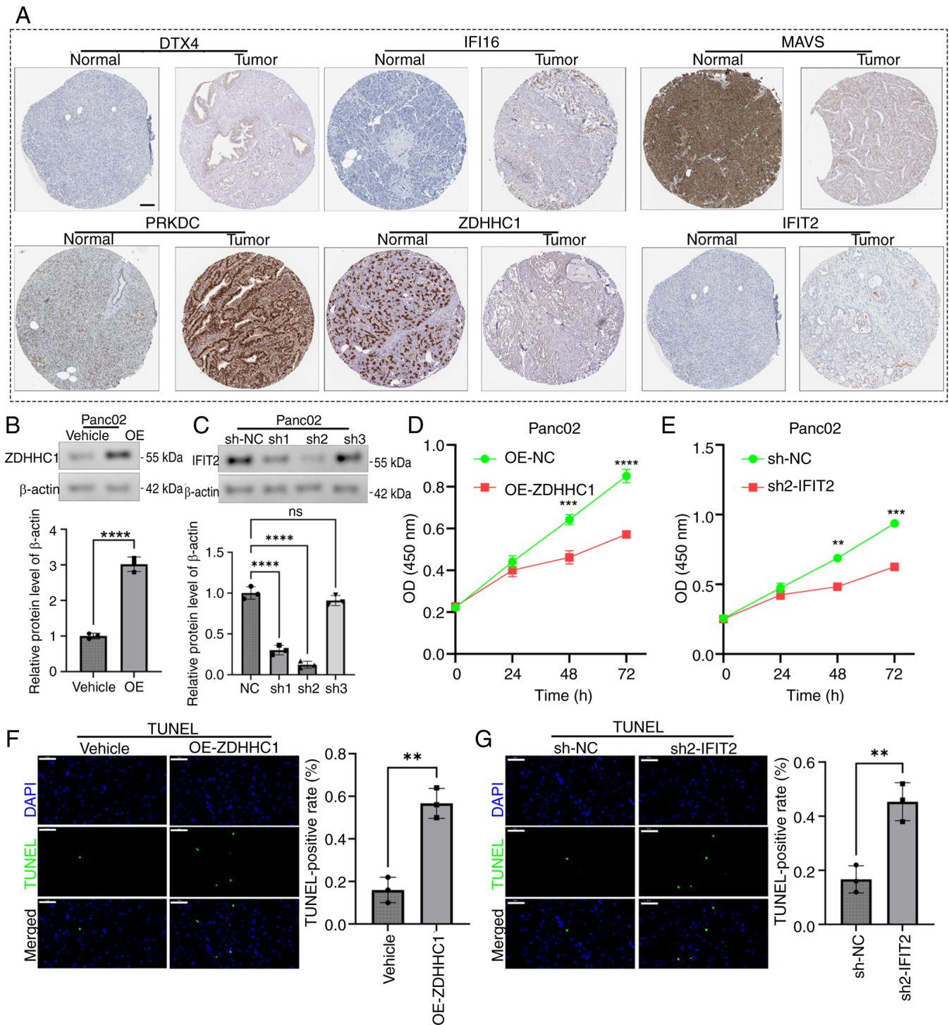
Figure 7. Functional roles of IFIT2 and ZDHHC1 in PAAD oncobiology. (A) Human Protein Atlas representative immunohistochemical staining of six prognostic signature genes in PAAD tissues (proteintlas.org). Scale bar, 100 \mu m. (B) Western blot and semi-quantification confirming successful ZDHHC1 overexpression in Panc02 cells (C) Western blot and semi-quantification confirming IFIT2 knockout efficiency in Panc02 cells (**** P <0.0001). (D) CCK-8 assay: ZDHHC1 overexpression enhances Panc02 proliferation (*** P <0.001 and **** P <0.0001 vs OE-NC). (E) CCK-8 assay: IFIT2 knockout enhances Panc02 proliferation (** P <0.01 and *** P <0.001 vs. sh-NC). (F) TUNEL assay (scale bar, 50 \mu m) demonstrating reduced apoptosis in ZDHHC1-overexpressing Panc02 cells. (G) TUNEL assay (scale bar 50 \mu m) showing decreased apoptosis in IFIT2-knockout Panc02 cells (** P <0.01). IFIT2, interferon-induced protein with tetratricopeptide repeats 2; ZDHHC1, zinc finger DHHC-type containing 1; PAAD, pancreatic ductal adenocarcinoma; OE, overexpression; CCK-8, Cell Counting Kit-8; DTX4, deltex E3 ubiquitin ligase 4; IFI16, interferon \gamma inducible protein 16; MAVS, mitochondrial antiviral-signaling protein; PRKDC, protein kinase DNA-activated catalytic subunit; sh-NC, scrambled negative control shRNA; ns, not significant.
