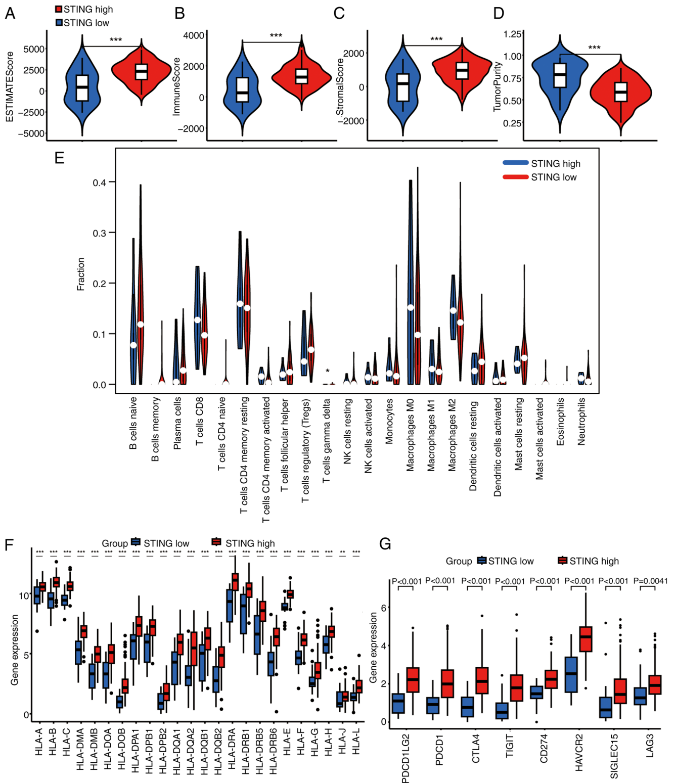
Figure 4. Immune microenvironment profiling of PAAD molecular subtypes. (A) ESTIMATE analysis showing significantly higher immune scores in STING1-high subtype (C1) vs. STING1-low subtype (C2). (B) Significantly higher immune scores in C1 vs. C2. (C) Significantly higher stromal scores in C1 vs. C2. (D) CIBERSORT analysis revealing differential immune cell infiltration patterns between subtypes (key immune subsets labeled) (***P<0.001). (E) Positive correlation between STING1 expression and \gamma\delta T cell infiltration density (Pearson r=0.68 ; *P<0.05). (F) Upregulated HLA molecule expression in C1 vs. C2 (**P<0.05 and ***P<0.01). (G) Elevated immune checkpoint molecule expression in C1 vs. C2. PAAD, pancreatic ductal adenocarcinoma; STING, stimulator of interferon genes; HLA, human leukocyte antigen; NK, natural killer.
