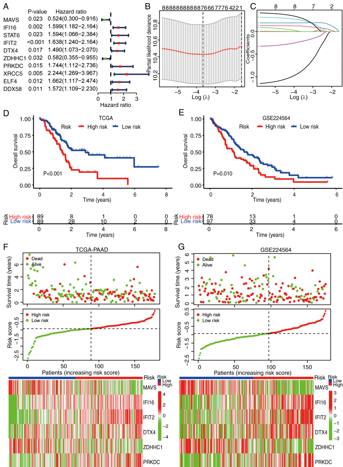
Figure 5. Development and validation of a STING1 signaling-related prognostic signature for PAAD. (A) Univariate Cox regression analysis of STING1 pathway-related genes in PAAD. Genes with significant prognostic value ( P < 0.05 ) are included. (B) LASSO regression 10-fold cross-validation curve showing optimal \lambda selection (minimum criteria). (C) LASSO coefficient profiles of STING1-related genes across log( \lambda ) sequence. (D) Kaplan-Meier survival analysis for the prognostic signature in TCGA-PAAD cohort (high-risk vs. low-risk groups; cutoff: median risk score). (E) Validation of prognostic signature in GSE224564 cohort. (F) Risk score distribution plot with corresponding survival status and expression heatmap for 6 signature genes in TCGA-PAAD. (G) Validation in GSE224564 cohort showing identical configuration to (F). STING, stimulator of interferon genes; PAAD, pancreatic ductal adenocarcinoma; LASSO, least absolute shrinkage and selection operator; TCGA, The Cancer Genome Atlas; MAVS, mitochondrial antiviral-signaling protein; IFI16, interferon \gamma inducible protein 16; IFIT2, interferon-induced protein with tetratricopeptide repeats 2; DTX4, deltex E3 ubiquitin ligase 4; ZDHHC1, zinc finger DHHC-type containing 1; PRKDC, protein kinase DNA-activated catalytic subunit; STAT6, signal transducer and activator of transcription 6; XRCC5, X-ray repair cross complementing; ELF4, E74-like ETS transcription factor 4; DDX58, RNA sensor RIG-I.
