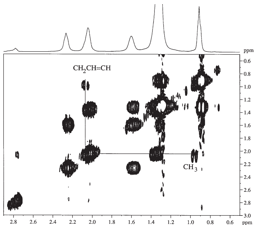
Figure 3. COSY spectrum of sample 2. The correlation \text{CH}_2\text{-CH}_3 of \alpha -linolenic acid is shown.
