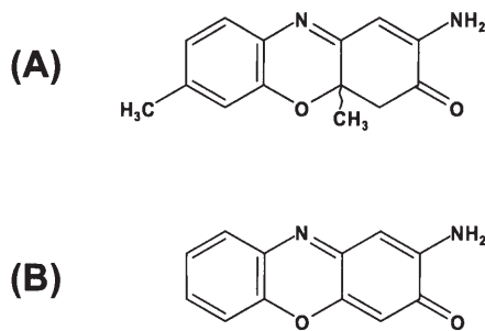
Figure 1. Chemical structure of the phenoxazine derivatives used in the present study. (A), 2-amino-4,4 \alpha -dihydro-4 \alpha ,7-dimethyl-3H-phenoxazine-3-one (Phx-1). (B), 2-aminophenoxazine-3-one (Phx-3).
