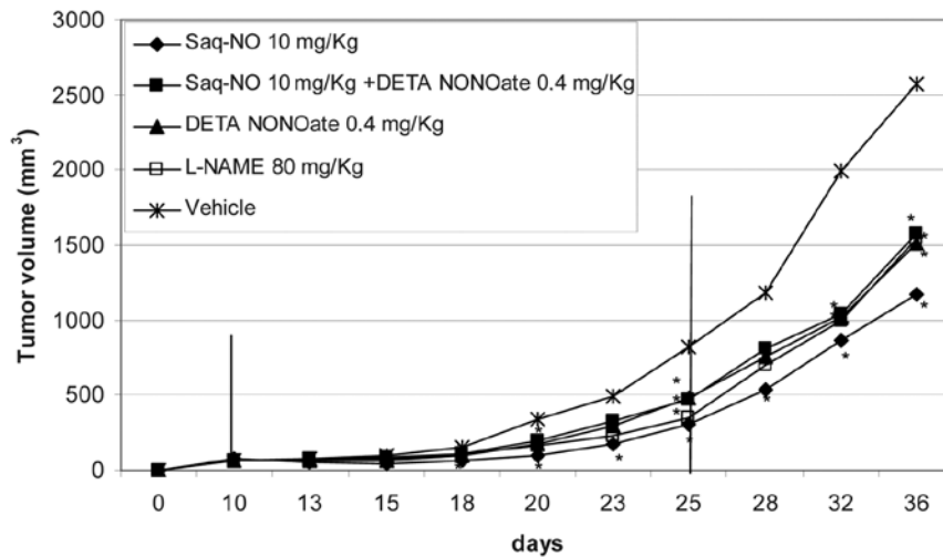
Figure 3. Saq-NO inhibited the growth of A375 melanoma cells in nude mice. Tumors were induced by subcutaneous implantation of 5 \times 10^6 A375 melanoma cells, and the compounds were injected intraperitoneally for 16 consecutive days starting on day 8-10 following tumor implantation. Tumor volumes were measured twice a week for 34-36 days after tumor implantation. Each group consisted of 8-11 mice. * p < 0.05 by t-test refers to vehicle-treated animals.
