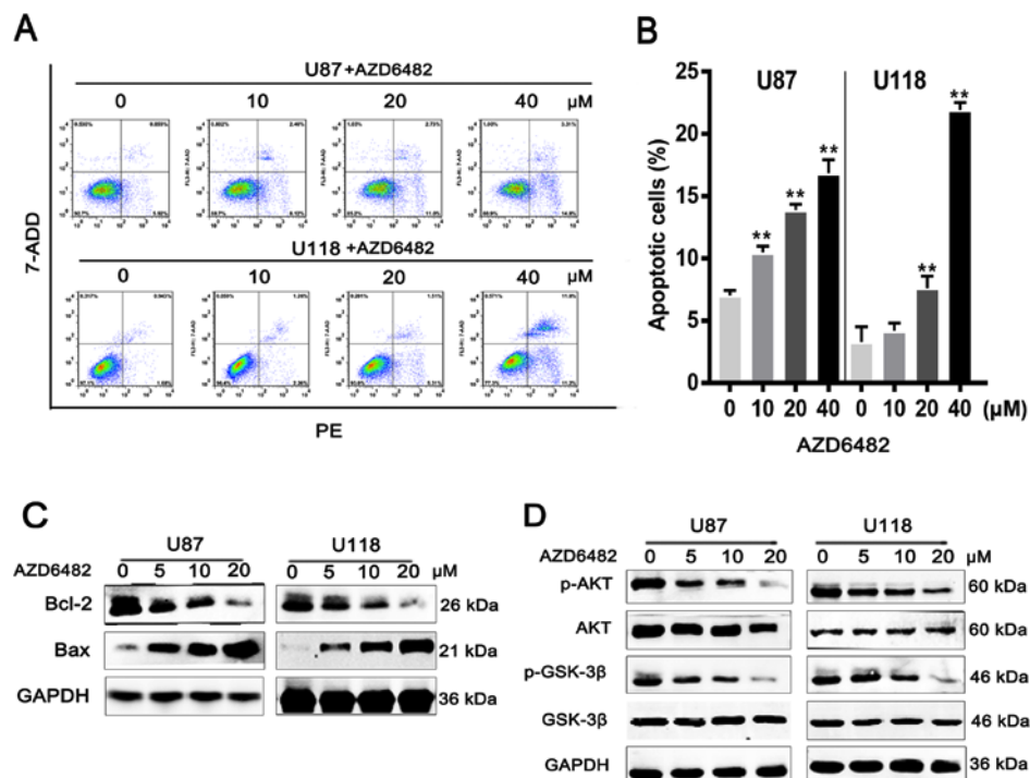
Figure 3. AZD6482 induces apoptosis in U87 and U118 cells. (A) U87 and U118 cells were treated with increasing concentrations of AZD6482 for 48 h, which was followed by an analysis of apoptosis by staining with 7-ADD/PE. (B) Apoptotic cells were measured by flow cytometry. ** P < 0.01 , compared with that of untreated controls (0 \mu\text{M} ). Data are presented as the mean \pm SD of at least three independent experiments. The expression levels of (C) Bcl-2, Bax and (D) related proteins of the PI3K signalling pathway were used to assess the inhibitory effect of AZD6482. Each protein was analysed in triplicate, and a representative experiment is shown.
