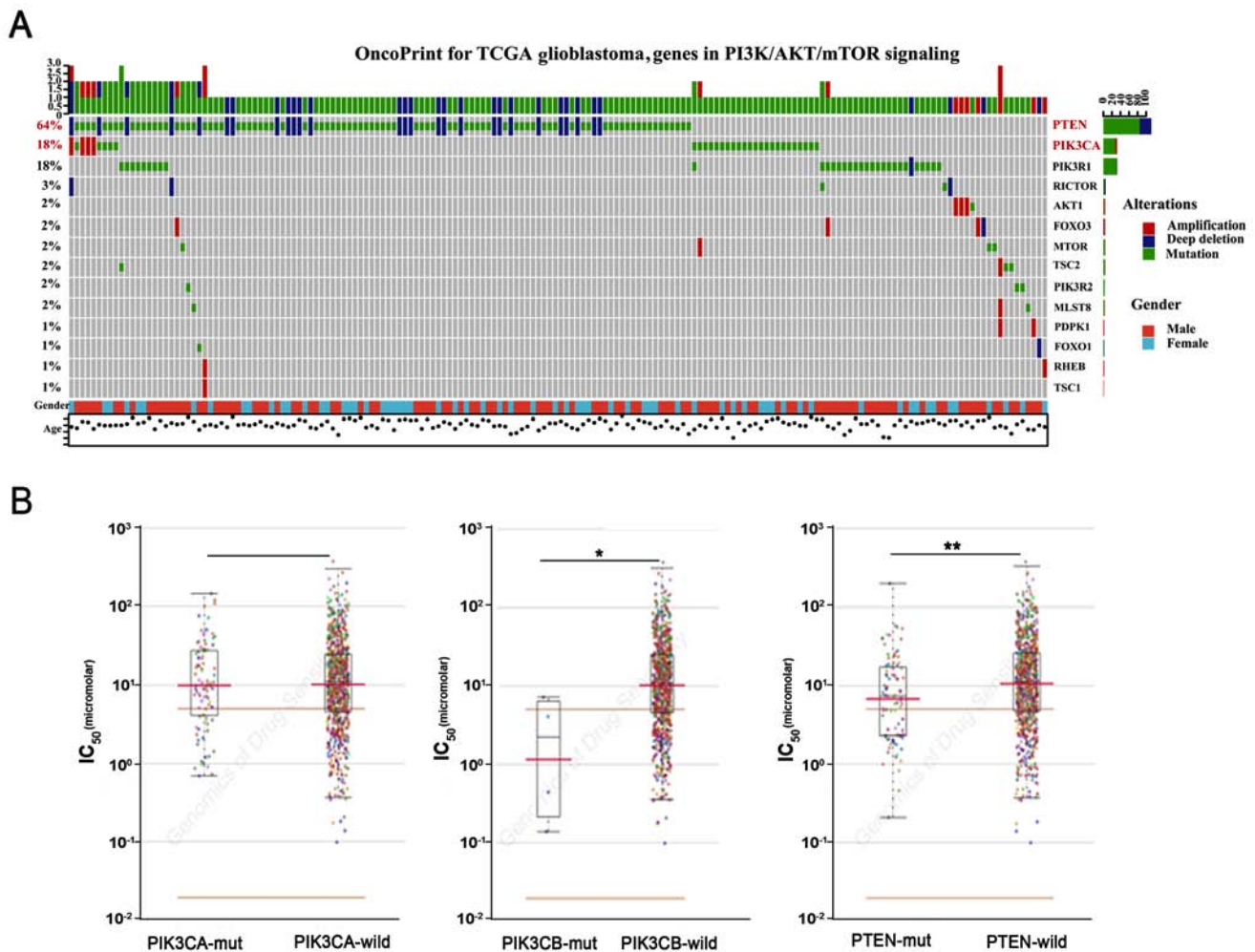
Figure 1. PTEN is frequently mutated in glioblastoma, and cancer cell lines with PTEN mutations were sensitive to AZD6482. (A) Mutation data of glioblastoma from The Cancer Genome Atlas (TCGA) database showed the genetic alteration status of the PI3K signalling pathway. (B) Data of GDSC database showed the relationship between various gene mutations and drug sensitivity. Scatter plot showed IC 50 values of PIK3CA-mutated, PIK3CB-mutated, PTEN-mutated and corresponding wild-type cell lines following treatment with AZD6482. Each point represents the IC 50 value for an individual cell line. The red lines indicate the geometric mean. The lower and upper lines indicated the minimum and maximum concentration of AZD6482. Mut, mutated; wild, wild-type. *P<0.05, **P<0.01
