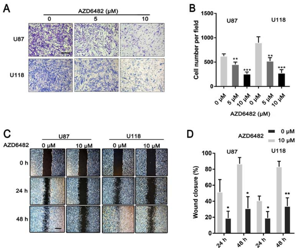
Figure 5. AZD6482 inhibits glioblastoma cell migration and invasion. (A) The invasion ability of U87 and U118 gradually decreased with increasing concentrations of AZD6482. Scale bar, 100 \mu m. (B) The invaded cells were counted under a light microscope. (C) The cell monolayer was wounded with a pipette tip and treated with 0 or 10 \mu M AZD6482. Images were acquired at 0, 24, and 48 h in the wound-healing assay. Scale bar, 500 \mu m. (D) The rate of wound closure in the AZD6482-treated group was lower than that in the untreated group at 48 h of growth. Data are presented as the means \pm SD of three independent experiments; * P <0.05, ** P <0.01, *** P <0.001, compared with the untreated controls (0 \mu M).
