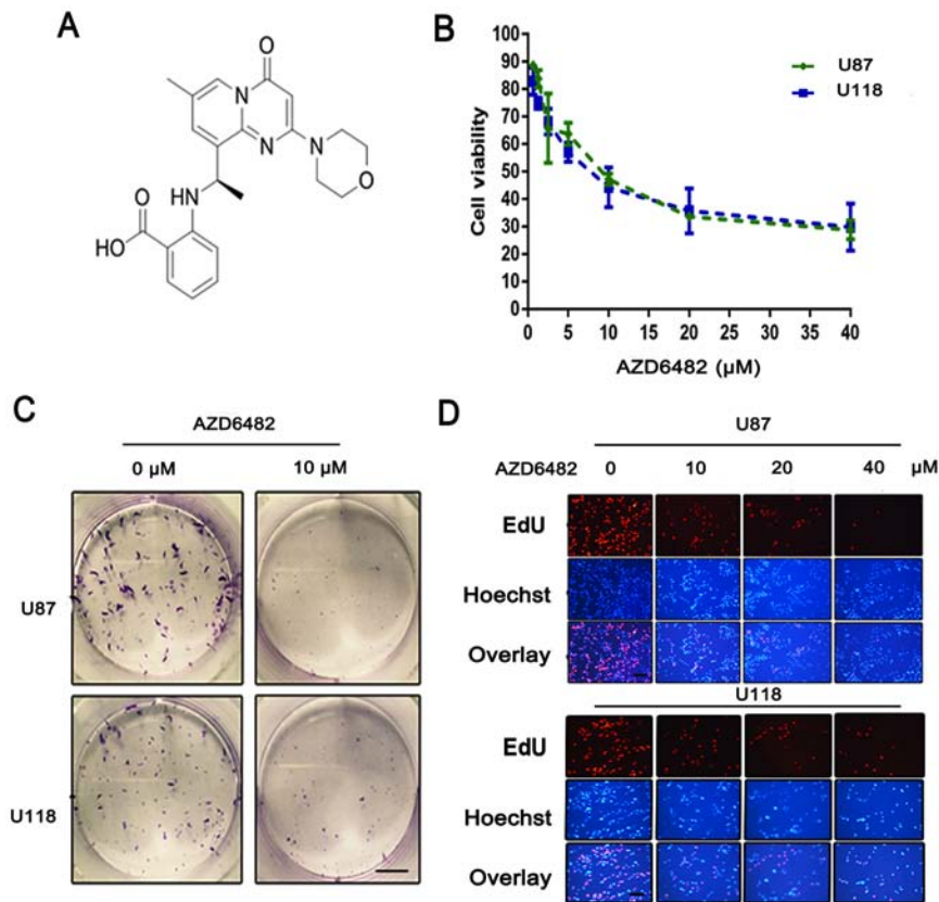
Figure 2. Treatment with AZD6482 leads to an anti-proliferative effect on glioblastoma cells. (A) The molecular structure of AZD6482. (B) Cell viability was determined by CCK-8 assay after AZD6482 treatment at various concentrations (0, 0.625, 1.25, 2.5, 5, 10, 20, or 40 \mu\text{M} ) for 48 h. Each cell line was analysed in triplicate. (C) AZD6482 inhibited the colony formation of U87 and U118 cells. Fewer colonies were formed in the treated group compared with the control group. Scale bar, 50 \mu\text{m} . (D) DNA replication activity was assessed by an EdU incorporation assay. Nuclei were stained with Hoechst (blue), and the proliferative cells were dyed red with EdU. Scale bar, 100 \mu\text{m} (same magnification in all panels).
