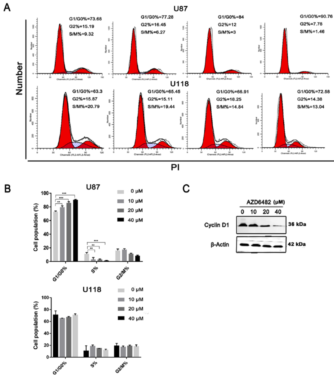
Figure 4. AZD6482 induces cell cycle arrest at the G1 phase in U87 cells. (A) Cell cycle distribution analysis by flow cytometry. AZD6482-induced G1 phase arrest in U87 cells after exposure to AZD6482 (0-40 μM) for 48 h. (B) The percentage of the cell population in G1/G0, S and G2/M phases. Data are presented as the mean ± SD of at least three independent experiments (n=3). **P<0.01, ***P<0.001, compared with the untreated controls (0 μM). (C) The effects of AZD6482 on the expression of cyclin D1 are presented by western blot analysis.
