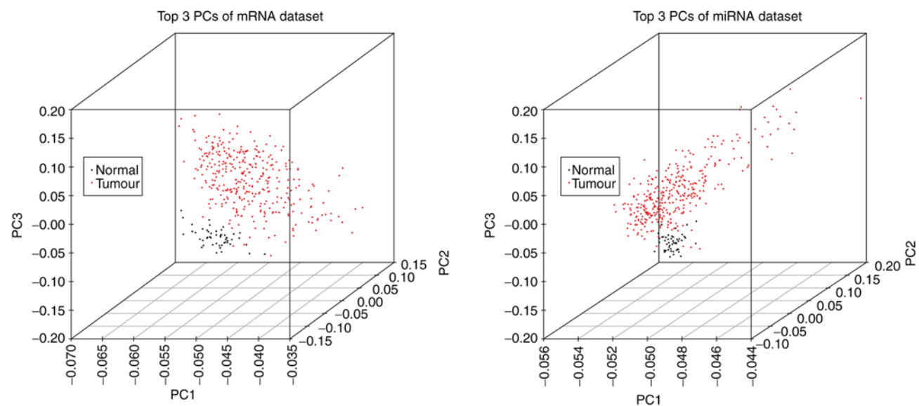
Figure S1. PC analysis of miRNAs and mRNAs in hepatocellular carcinoma. miR, microRNA; PC, principal component.
