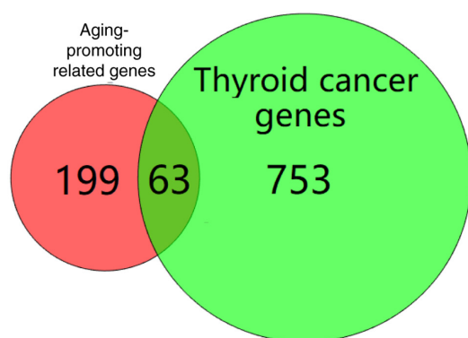
Figure S1. Venn diagram of the genes associated with both age-promotion and thyroid cancer.
