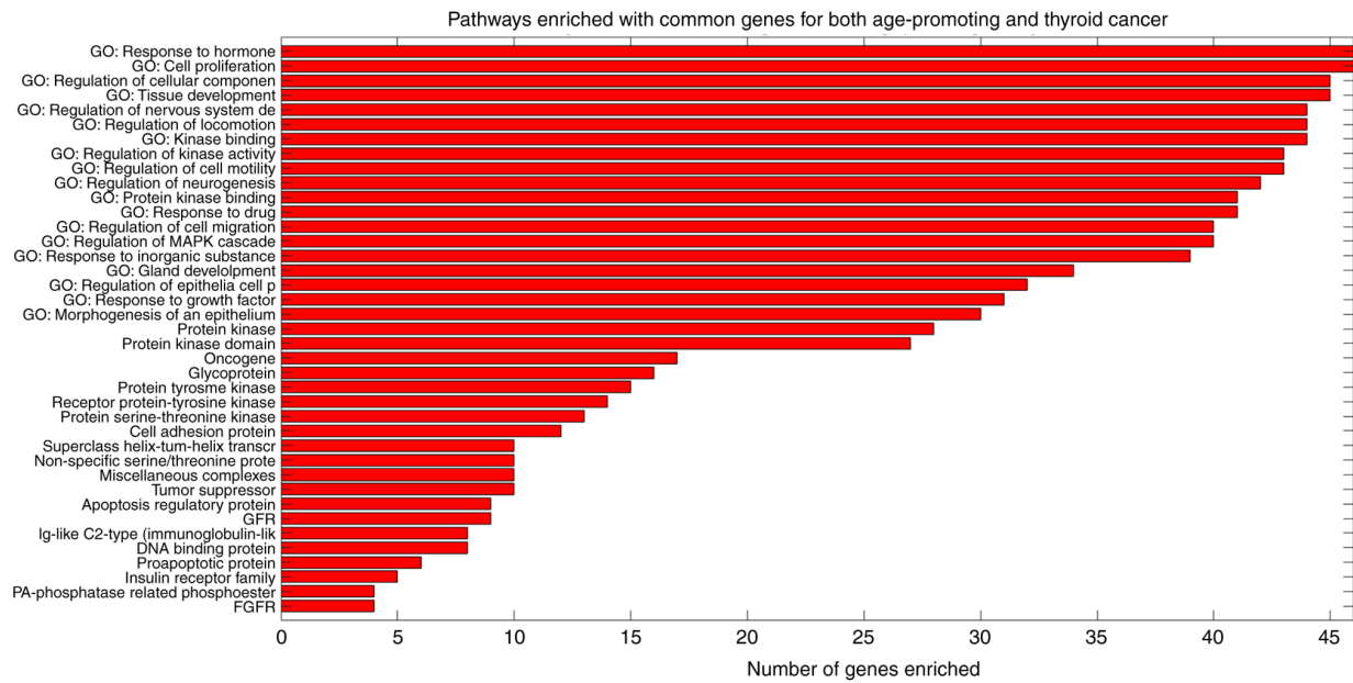
Figure S2. Significant pathways from gene set enrichment analysis results.
