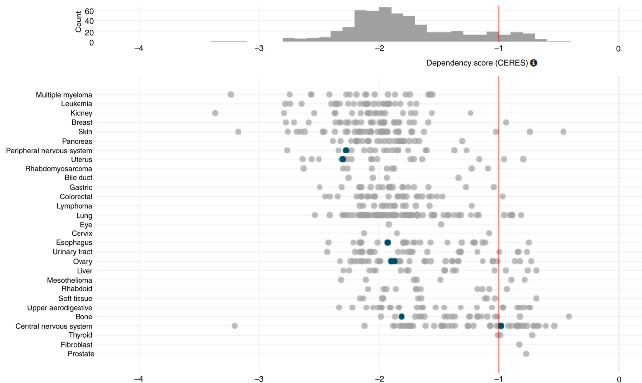
Figure S1. Depmap analysis indicated that knockout of yrdC N6-threonylcarbamoyltransferase domain containing protein could significantly suppress the growth of several non-small cell lung carcinoma cell lines. Grey dots represent wild type cell lines and blue dots represent cell lines with mutated genes.
