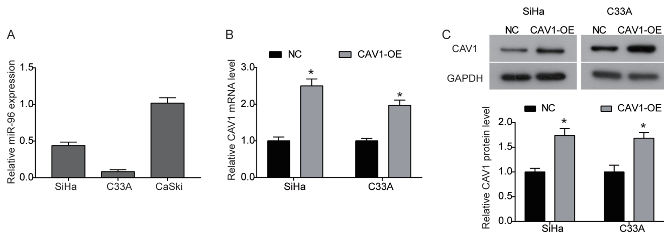
Figure S1. Expression levels of miR-96 and CAV-1 in cervical cancer cell lines. (A) Expression level of miR-96 in SiHa, C33A and CaSki cells. (B) Expression level of CAV-1 mRNA in SiHa and C33A cells transfected with pcDNA3.1-CAV-1 vector. (C) Protein expression level of CAV-1 in SiHa and C33A cells transfected with pcDNA3.1-CAV-1 vector. * P < 0.05 . Data are presented as the mean \pm SD. miR-96, microRNA-96; CAV-1, caveolin 1; CAV-1-OE, cells transfected with pcDNA3.1-CAV-1 overexpression vector; NC, negative control.
