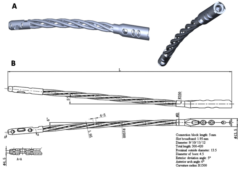
Figure S1. (A) Geometric structure and (B) specific parameters of the novel intramedullary nail.
