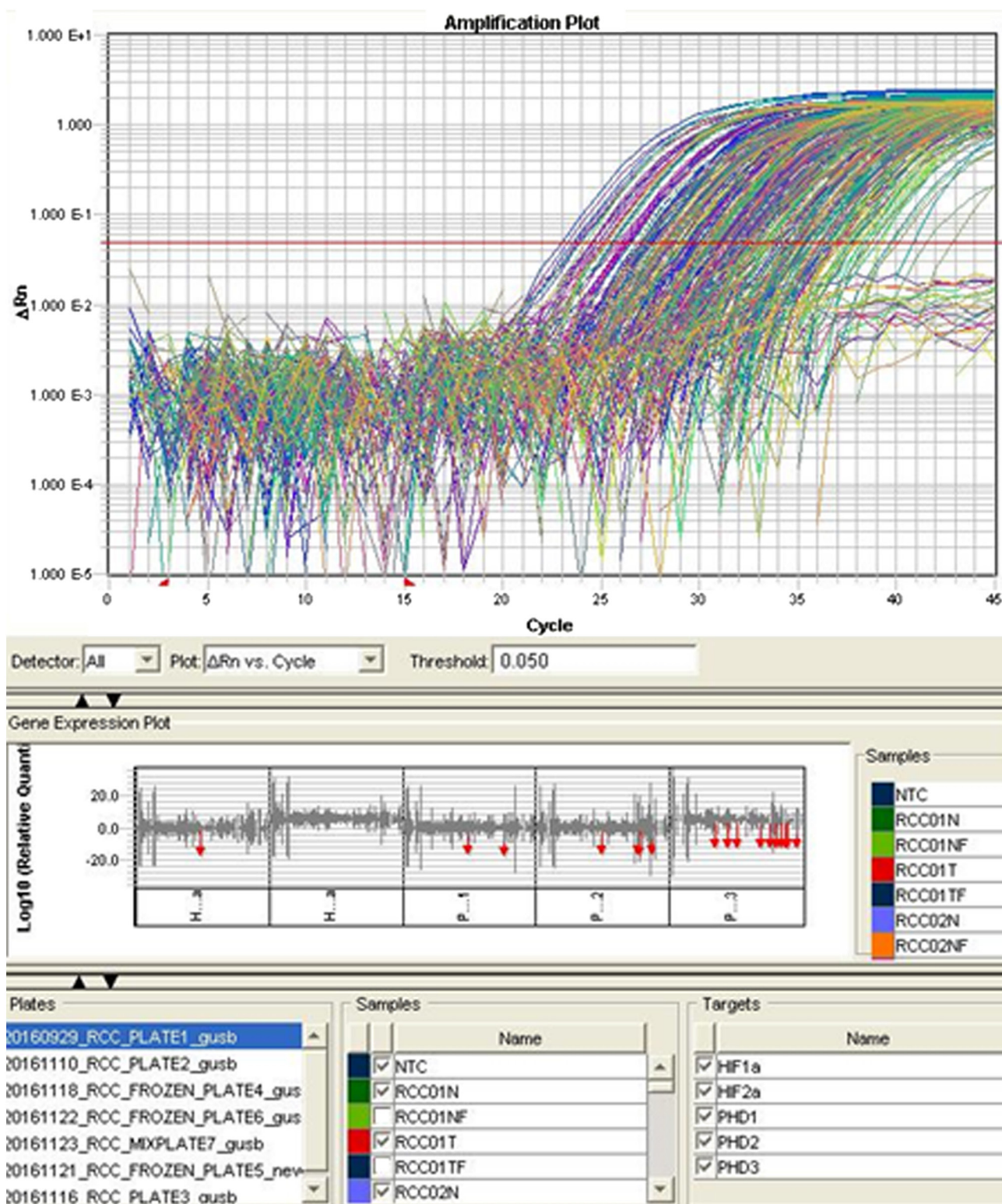
Figure S1. Amplification plots of formalin-fixed paraffin-embedded samples (tumour and normal) included in one run for all markers. Samples with Ct values \geq 36 were excluded from the analysis.
