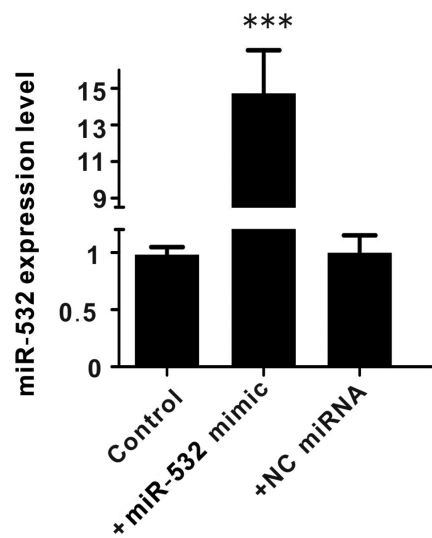
Figure S1. Expression of miR-532-3p in SH-SY5Y cells. +miR-532-3P mimics, cells treated with miR-532-3P mimic (50 \mu M); +NC miRNA, cells with negative control miRNA (50 \mu M). Data are presented as the mean \pm standard deviation. ***P<0.001 vs. control. NC, negative control; miR/miRNA, microRNA.
