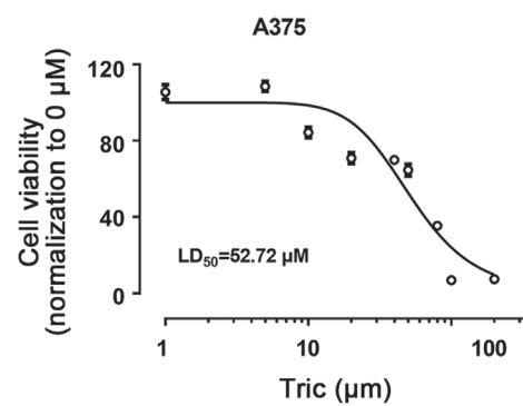
Figure S1. LD 50 of triclosan in A375 melanoma cells.
